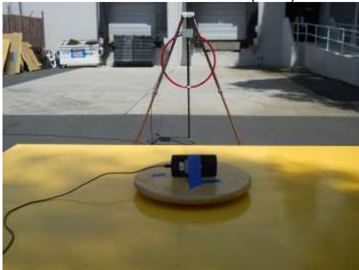
RADIATED EMISSIONS BELOW 30MHz (BACK)
