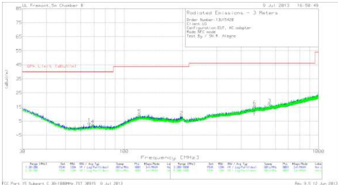
EMI PLOT
