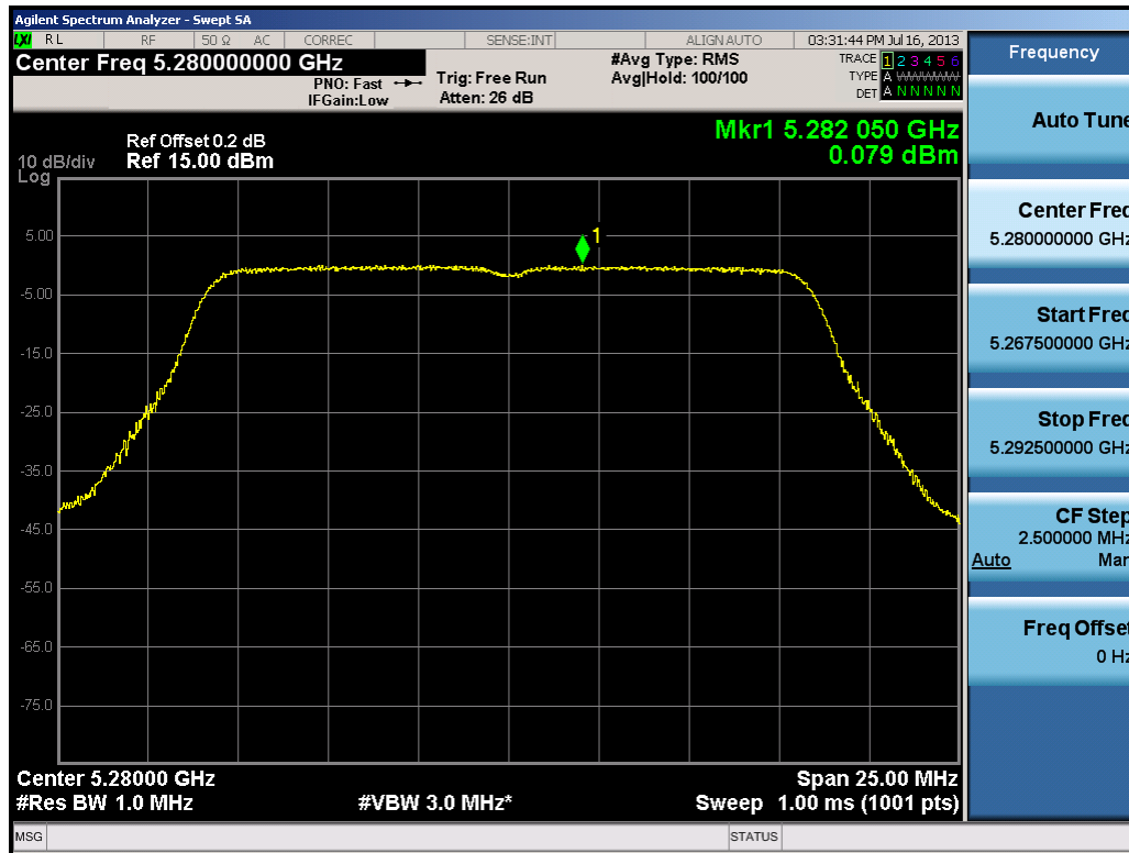
Plot 6-52. Peak Power Spectral Density Plot (802.11a (UNII Band 2) – Ch. 56)
