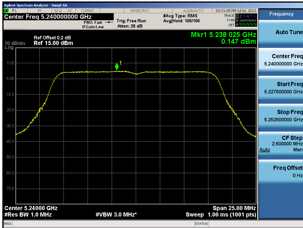
Plot 6-44. Peak Power Spectral Density Plot (802.11a (UNII Band 1) – Ch. 48)
