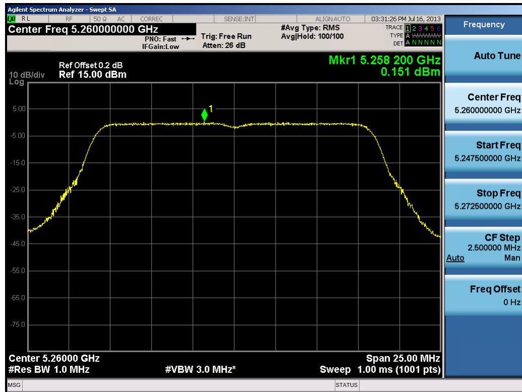
Plot 6-51. Peak Power Spectral Density Plot (802.11a (UNII Band 2) – Ch. 52)
