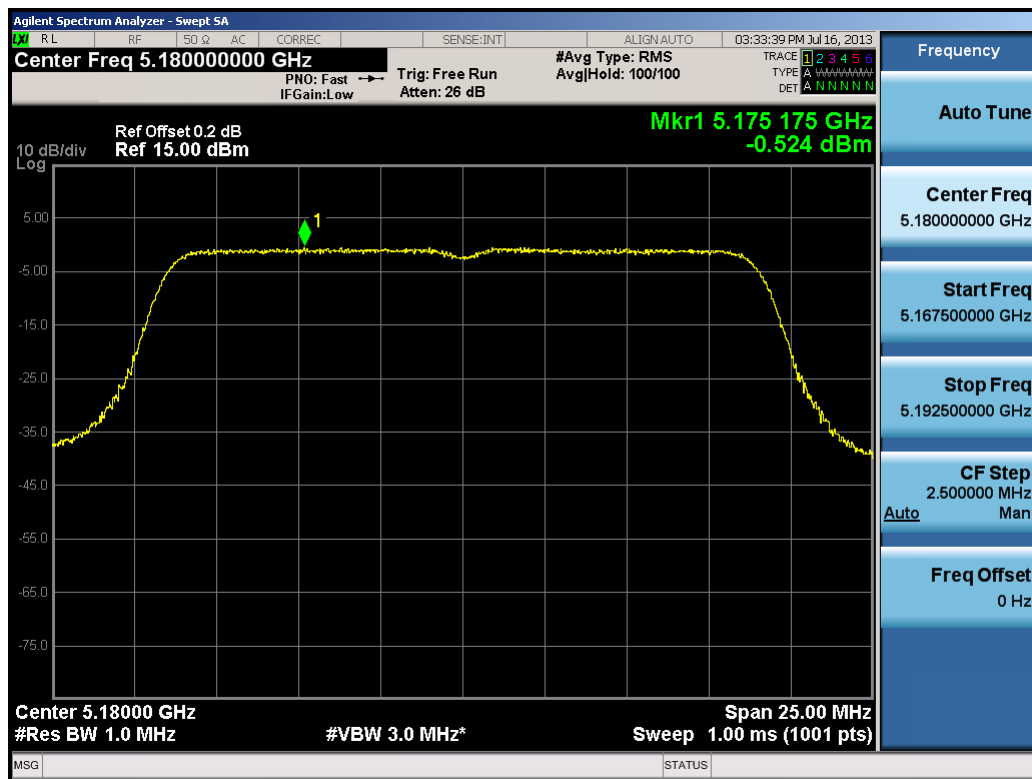
Plot 6-45. Peak Power Spectral Density Plot (20MHz BW 802.11n (UNII Band 1) – Ch. 36)
