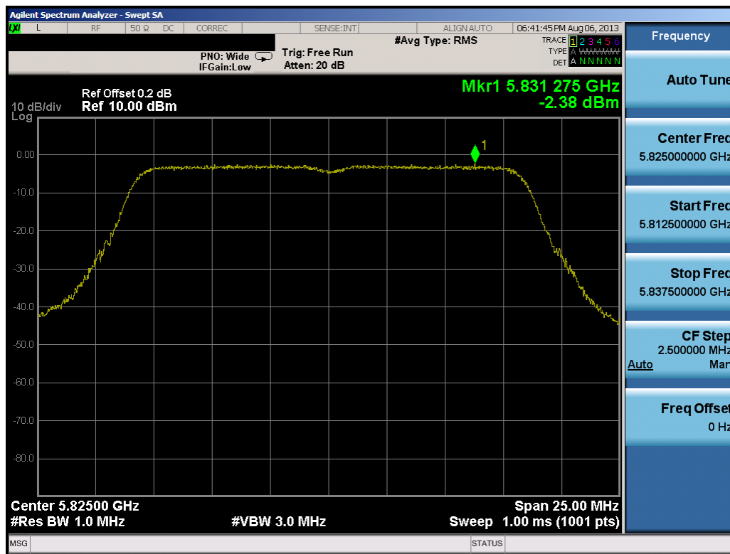
Plot 6-73. Peak Power Spectral Density Plot (20MHz BW 802.11a (UNII Band 4) – Ch. 165)
