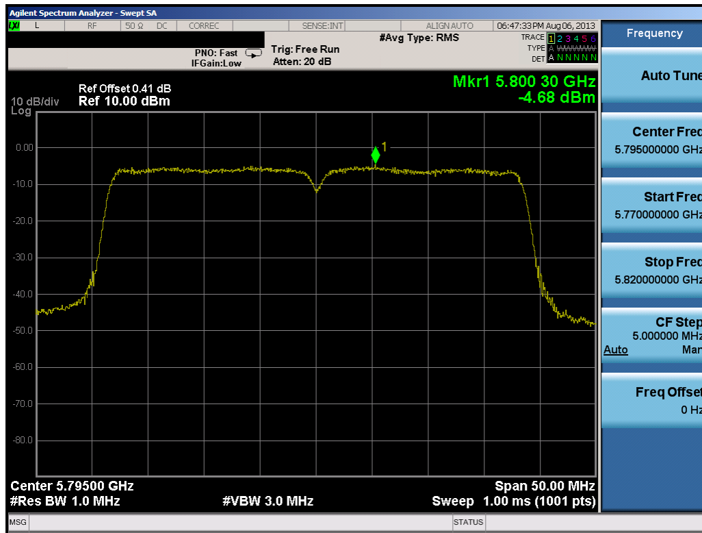
Plot 6-78. Peak Power Spectral Density Plot (40MHz BW 802.11n (UNII Band 4) – Ch. 159)
