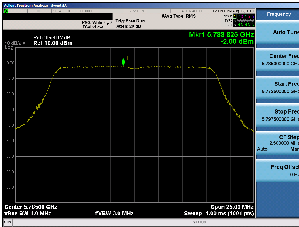
Plot 6-72. Peak Power Spectral Density Plot (20MHz BW 802.11a (UNII Band 4) – Ch. 157)
