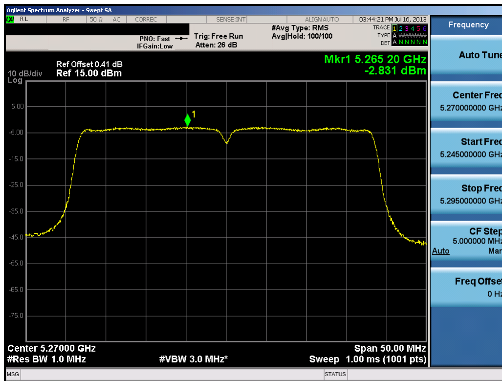
Plot 6-57. Peak Power Spectral Density Plot (40MHz BW 802.11n (UNII Band 2) – Ch. 54)
