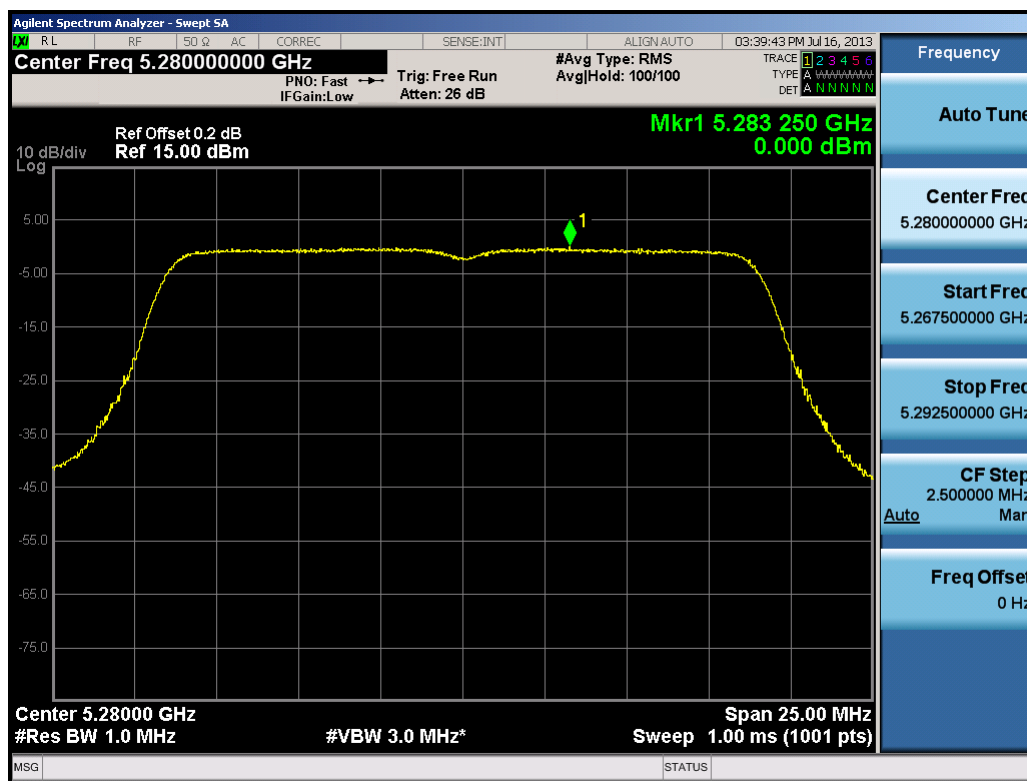
Plot 6-55. Peak Power Spectral Density Plot (20MHz BW 802.11n (UNII Band 2) – Ch. 56)
