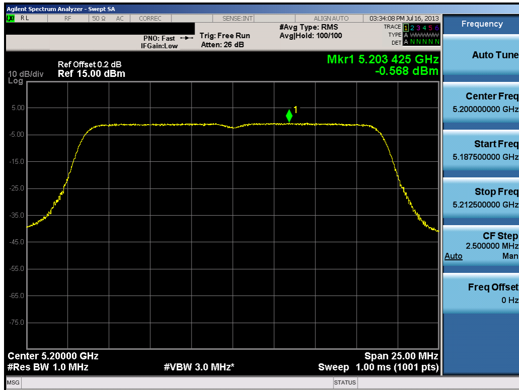
Plot 6-46. Peak Power Spectral Density Plot (20MHz BW 802.11n (UNII Band 1) – Ch. 40)
