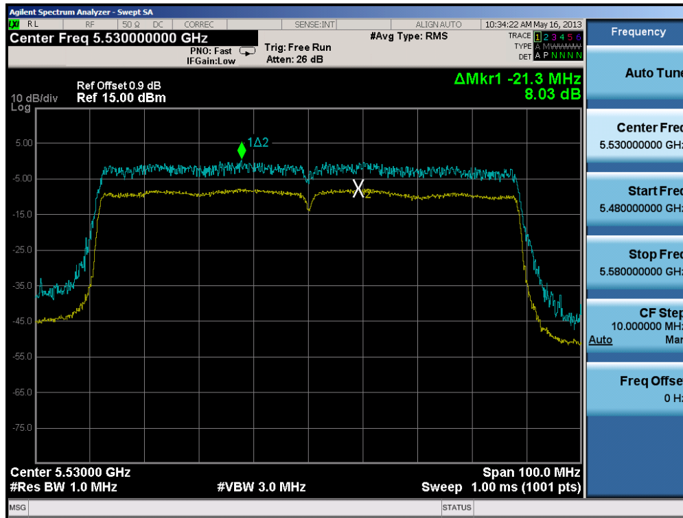
Plot 6-83. Peak Excursion Ratio Plot (80MHz BW 802.11ac)
