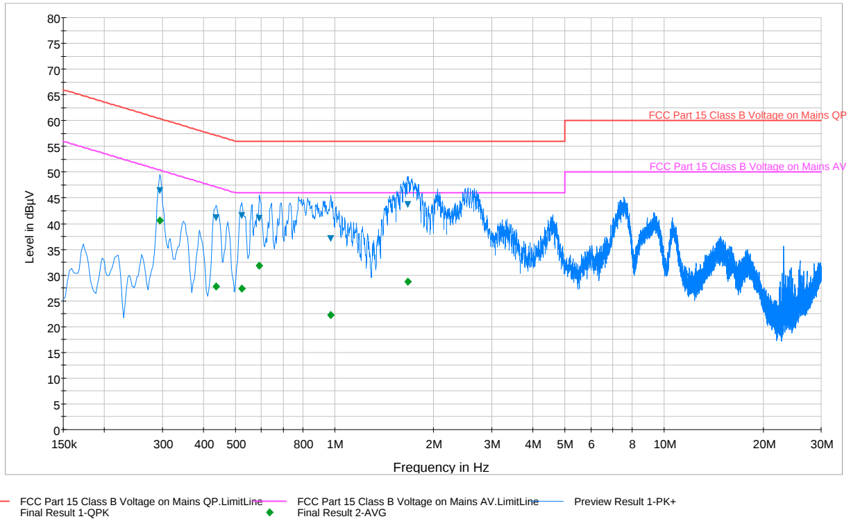
Plot 6-105. Line Conducted Plot with 802.11a UNII Band 1 (L1)
