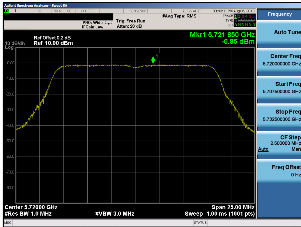
Plot 6-62. Peak Power Spectral Density Plot (802.11a (UNII Band 3) – Ch. 144)
