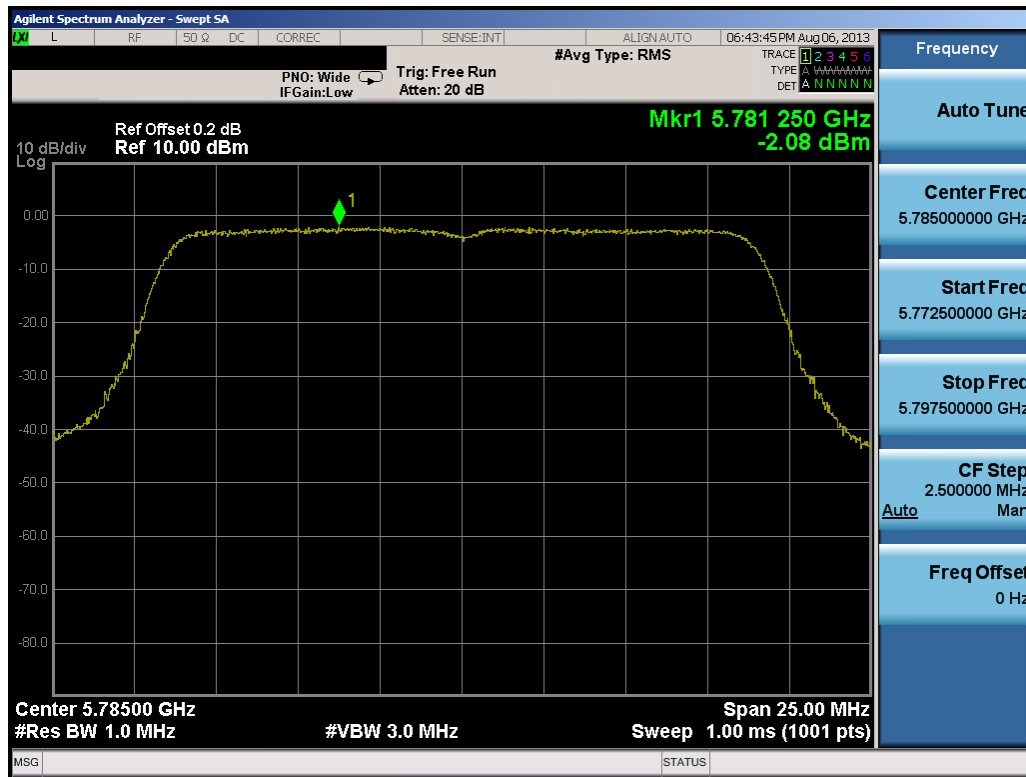
Plot 6-75. Peak Power Spectral Density Plot (20MHz BW 802.11n (UNII Band 4) – Ch. 157)
