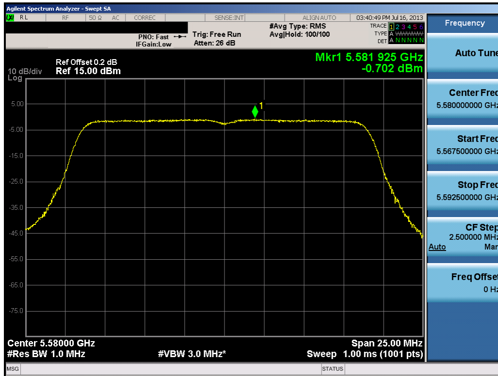
Plot 6-64. Peak Power Spectral Density Plot (20MHz BW 802.11n (UNII Band 3) – Ch. 116)
