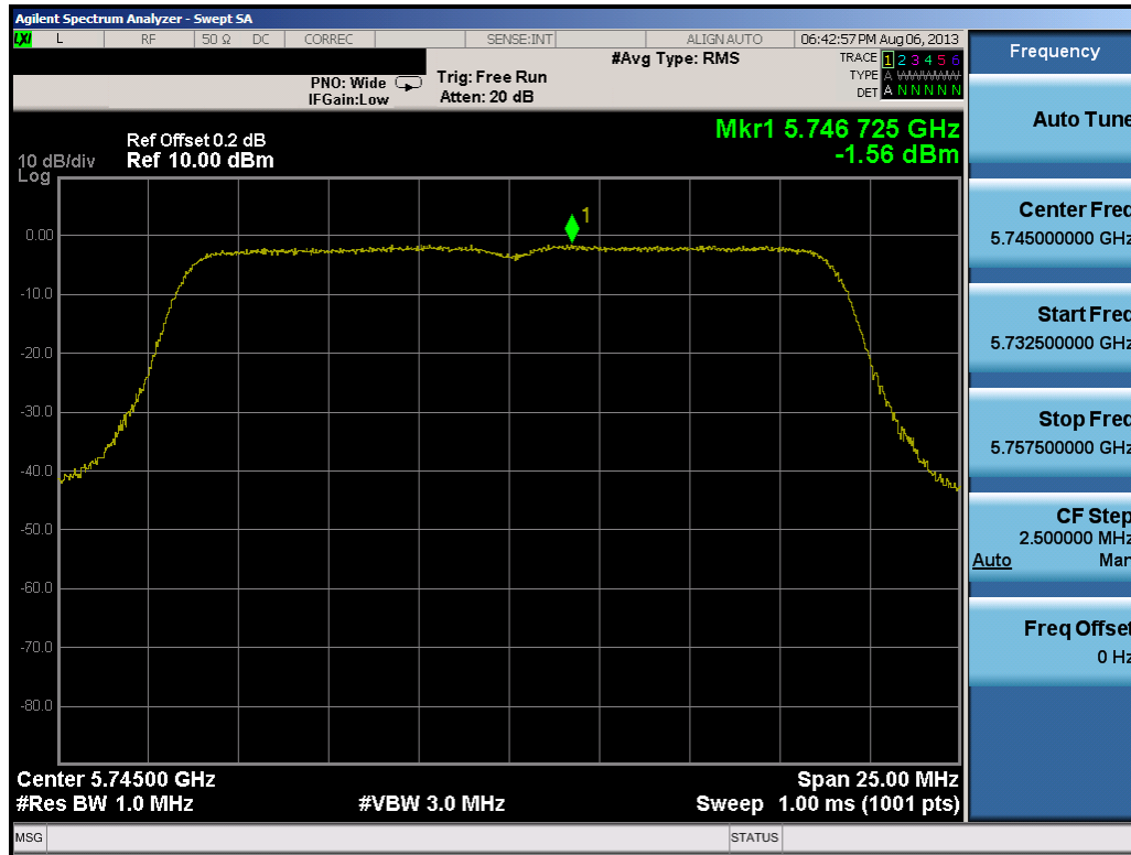
Plot 6-74. Peak Power Spectral Density Plot (20MHz BW 802.11n (UNII Band 4) – Ch. 149)
