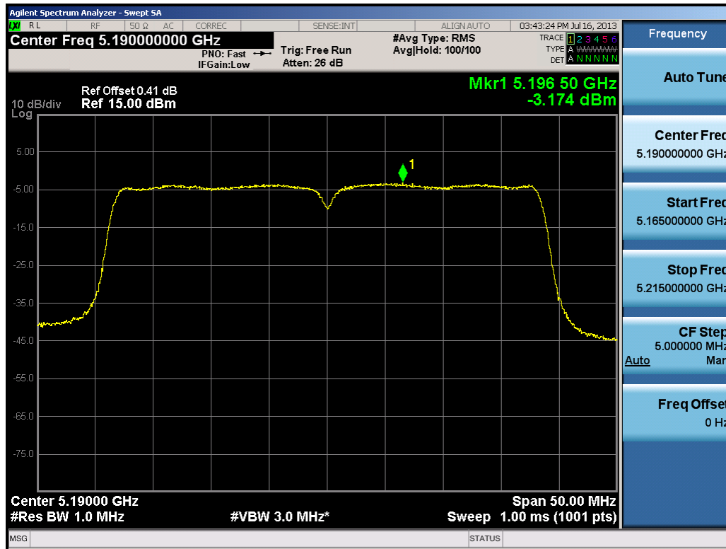
Plot 6-48. Peak Power Spectral Density Plot (40MHz BW 802.11n (UNII Band 1) – Ch. 38)
