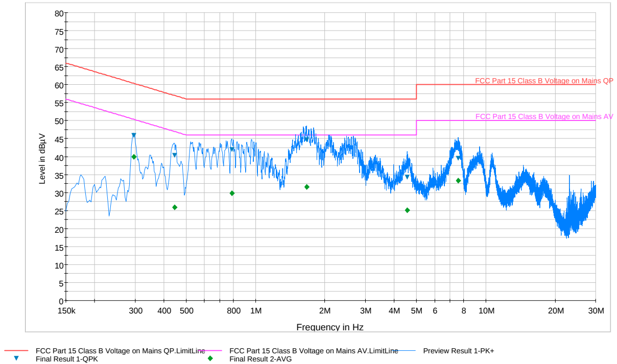
Plot 6-109. Line Conducted Plot with 802.11a UNII Band 3 (L1)
