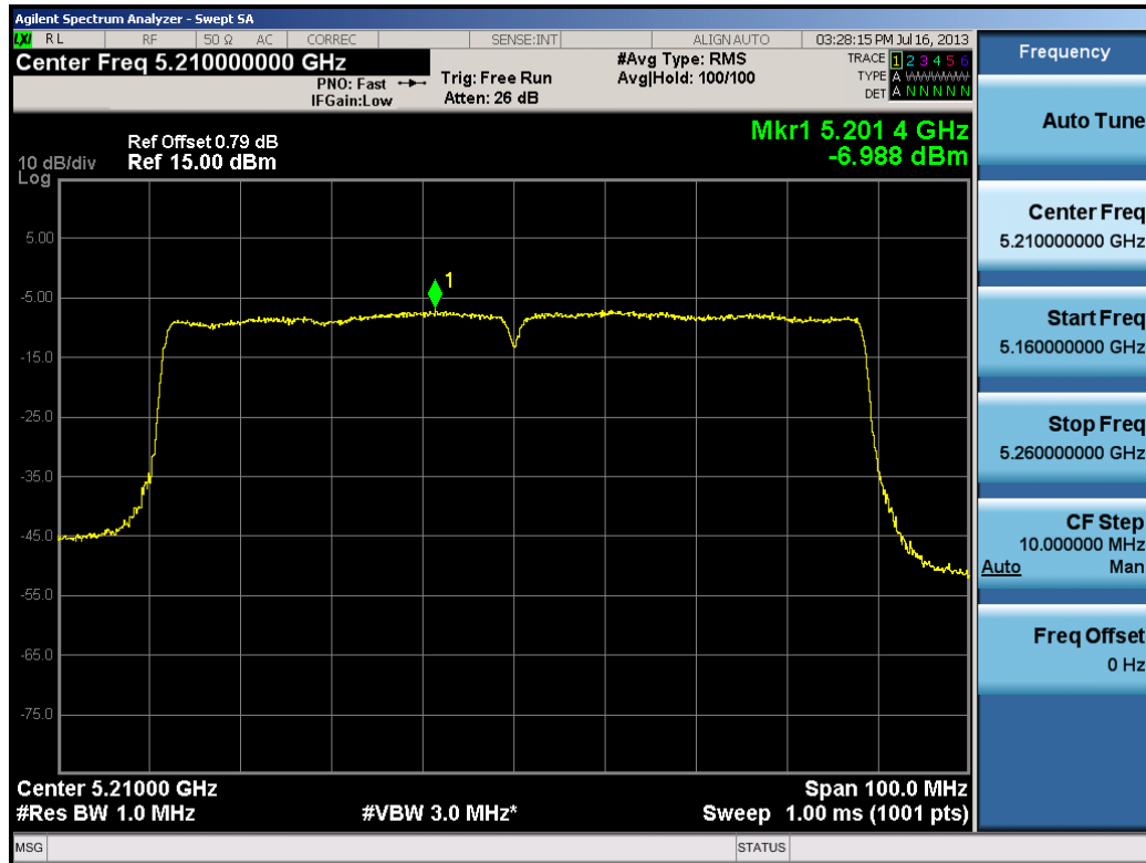
Plot 6-50. Peak Power Spectral Density Plot (80MHz BW 802.11ac (UNII Band 1) – Ch. 42)
