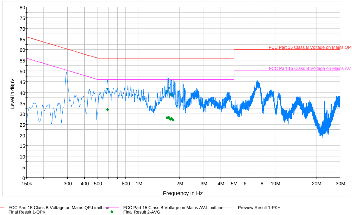
Plot 6-106. Line Conducted Plot with 802.11a UNII Band 1 (N)
