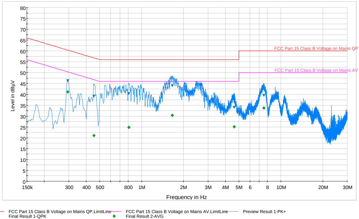
Plot 6-107. Line Conducted Plot with 802.11a UNII Band 2 (L1)
