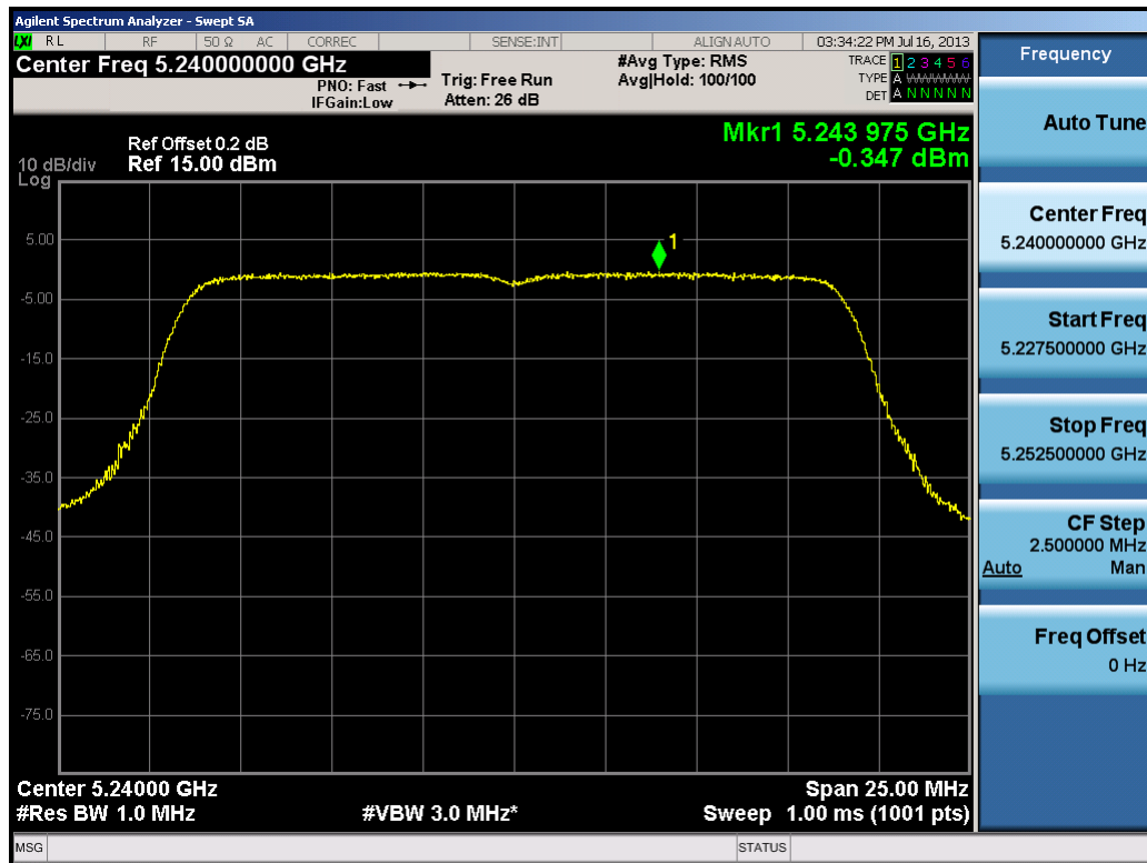
Plot 6-47. Peak Power Spectral Density Plot (20MHz BW 802.11n (UNII Band 1) – Ch. 48)
