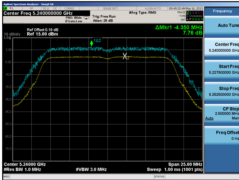
Plot 6-80. Peak Excursion Ratio Plot (802.11a)
