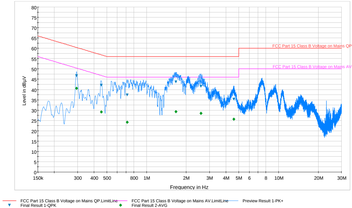
Plot 6-111. Line Conducted Plot with 802.11a UNII Band 4 (L1)
