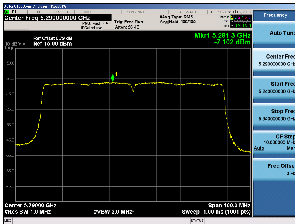
Plot 6-59. Peak Power Spectral Density Plot (80MHz BW 802.11ac (UNII Band 2) – Ch. 58)
