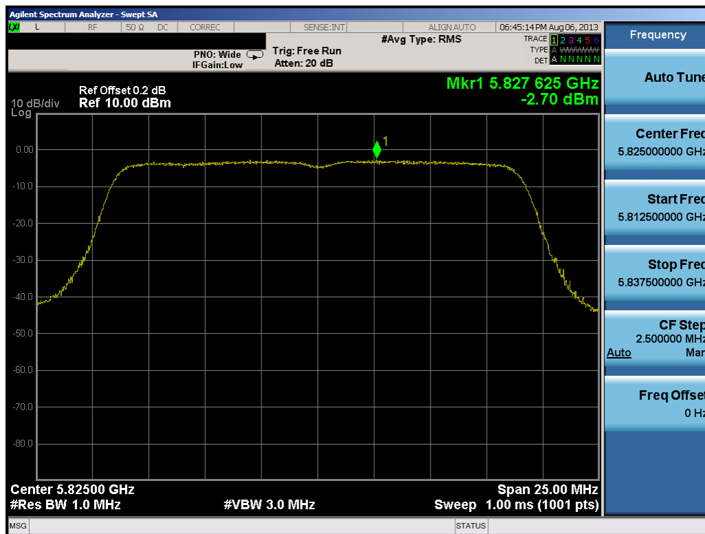
Plot 6-76. Peak Power Spectral Density Plot (20MHz BW 802.11n (UNII Band 4) – Ch. 165)
