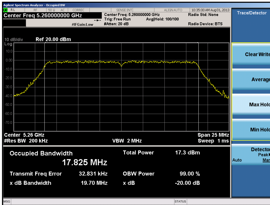
Plot 6-40. 20dB Bandwidth Plot (20MHz BW 802.11n (UNII Band 2) – Ch. 52)
