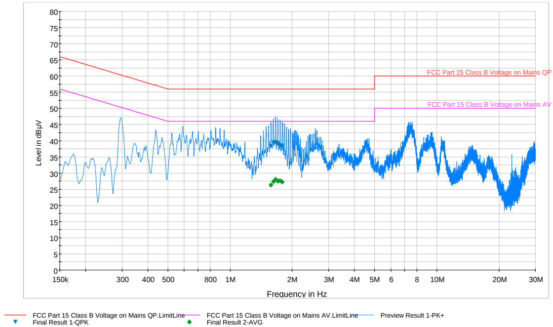
Plot 6-108. Line Conducted Plot with 802.11a UNII Band 2 (N)
