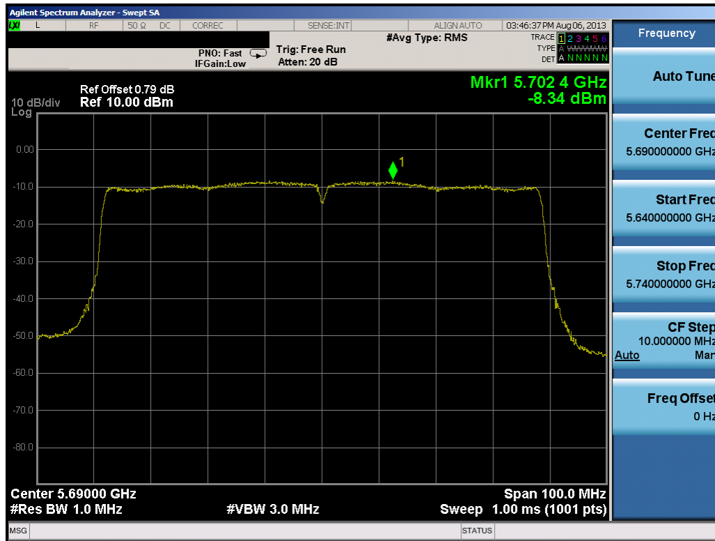
Plot 6-70. Peak Power Spectral Density Plot (80MHz BW 802.11ac (UNII Band 3) – Ch. 138)
