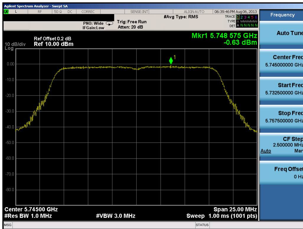
Plot 6-71. Peak Power Spectral Density Plot (20MHz BW 802.11a (UNII Band 4) – Ch. 149)
