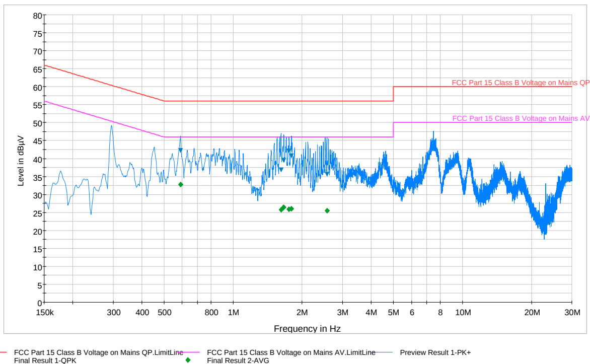
Plot 6-112. Line Conducted Plot with 802.11a UNII Band 4 (N)
