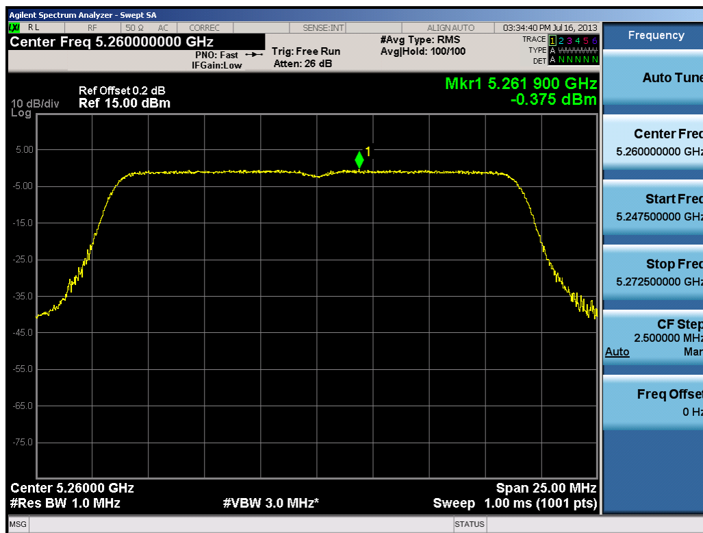
Plot 6-54. Peak Power Spectral Density Plot (20MHz BW 802.11n (UNII Band 2) – Ch. 52)
