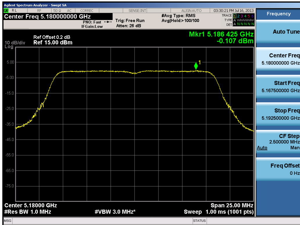
Plot 6-42. Peak Power Spectral Density Plot (802.11a (UNII Band 1) – Ch. 36)
