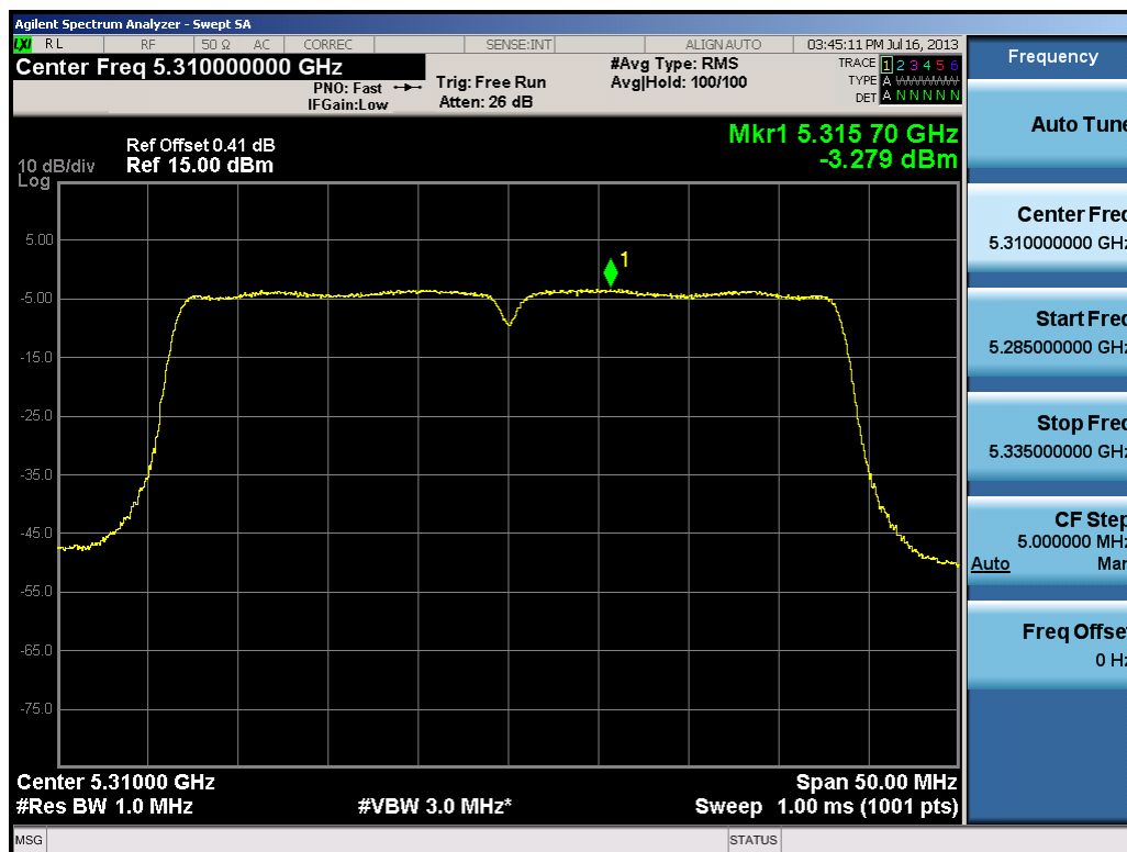
Plot 6-58. Peak Power Spectral Density Plot (40MHz BW 802.11n (UNII Band 2) – Ch. 62)
