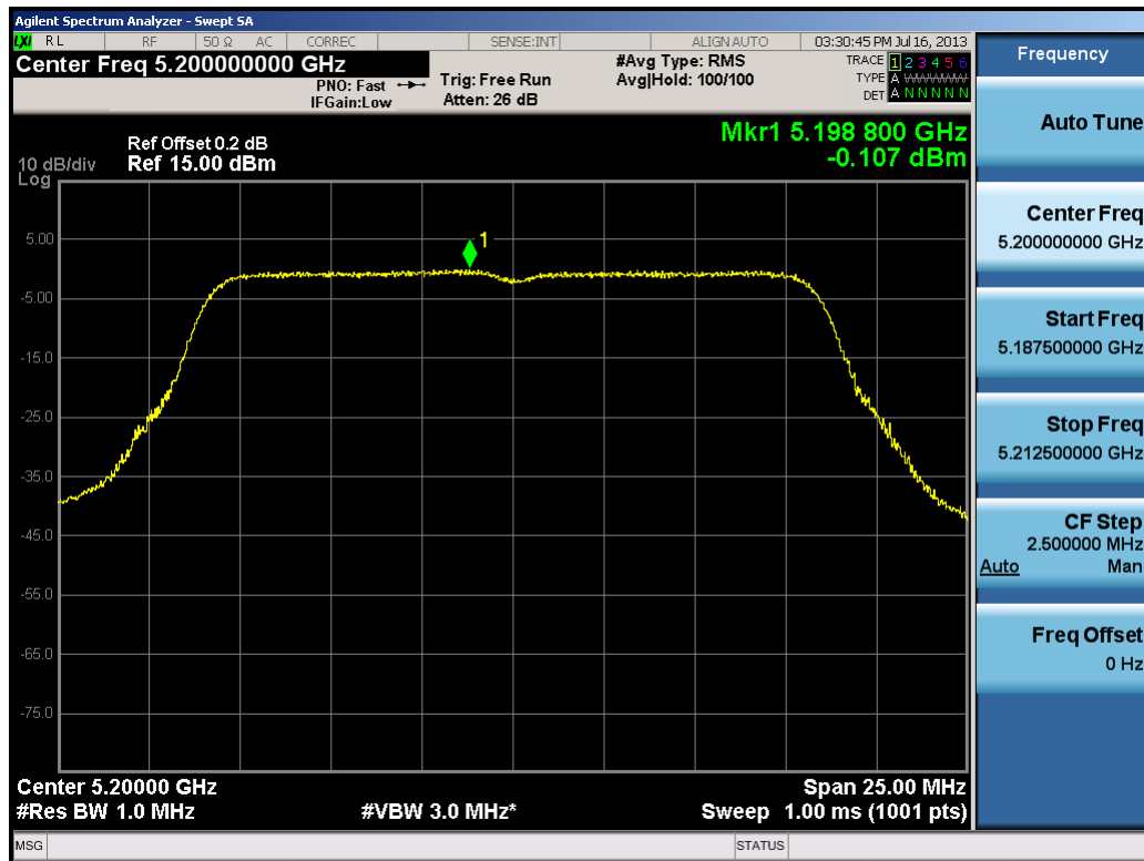
Plot 6-43. Peak Power Spectral Density Plot (802.11a (UNII Band 1) – Ch. 40)
