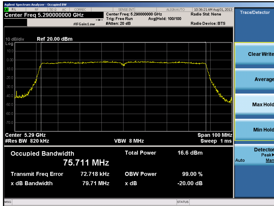
Plot 6-41. 20dB Bandwidth Plot (80MHz BW 802.11ac (UNII Band 2) – Ch. 58)
