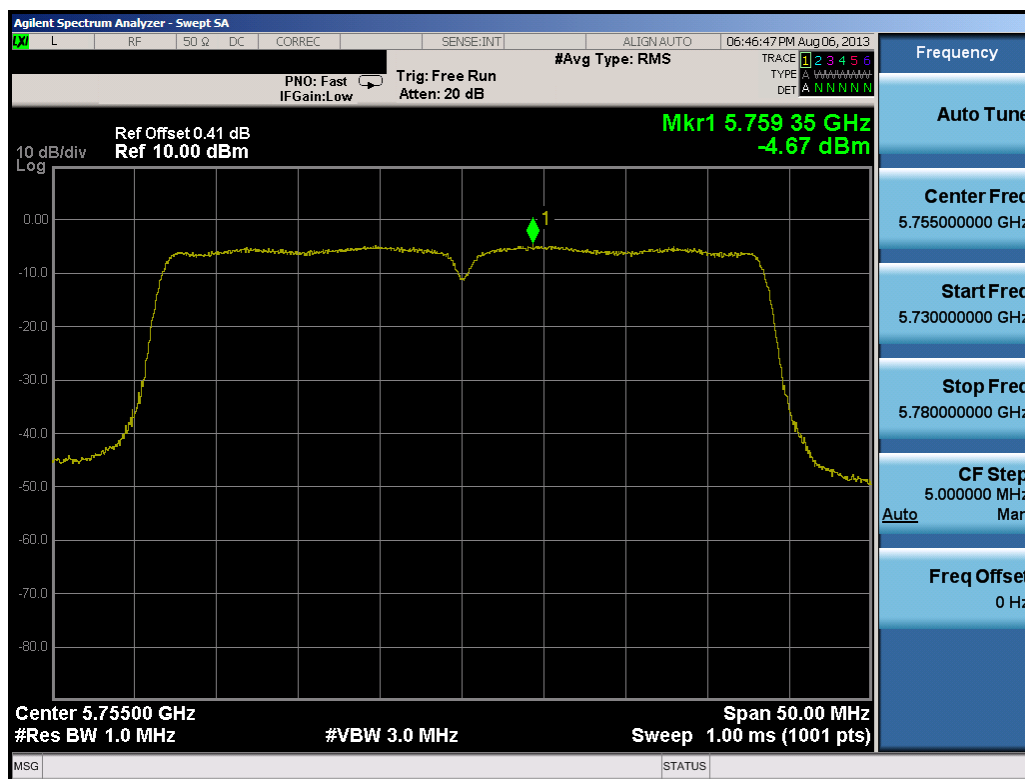
Plot 6-77. Peak Power Spectral Density Plot (40MHz BW 802.11n (UNII Band 4) – Ch. 151)
