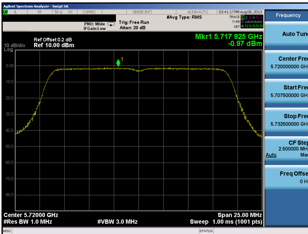
Plot 6-65. Peak Power Spectral Density Plot (20MHz BW 802.11n (UNII Band 3) – Ch. 144)
