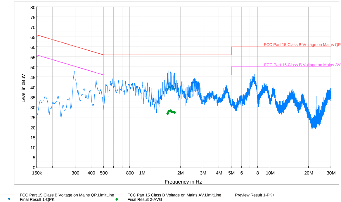
Plot 6-110. Line Conducted Plot with 802.11a UNII Band 3 (N)
