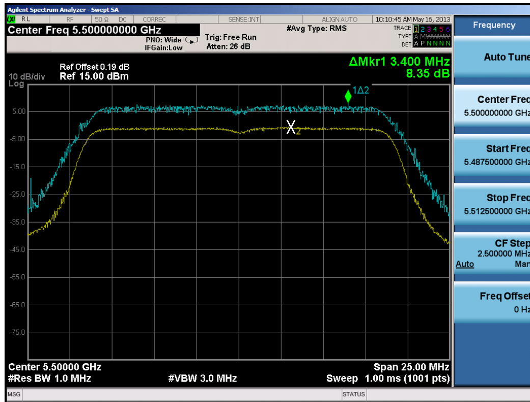
Plot 6-81. Peak Excursion Ratio Plot (20MHz BW 802.11n)
