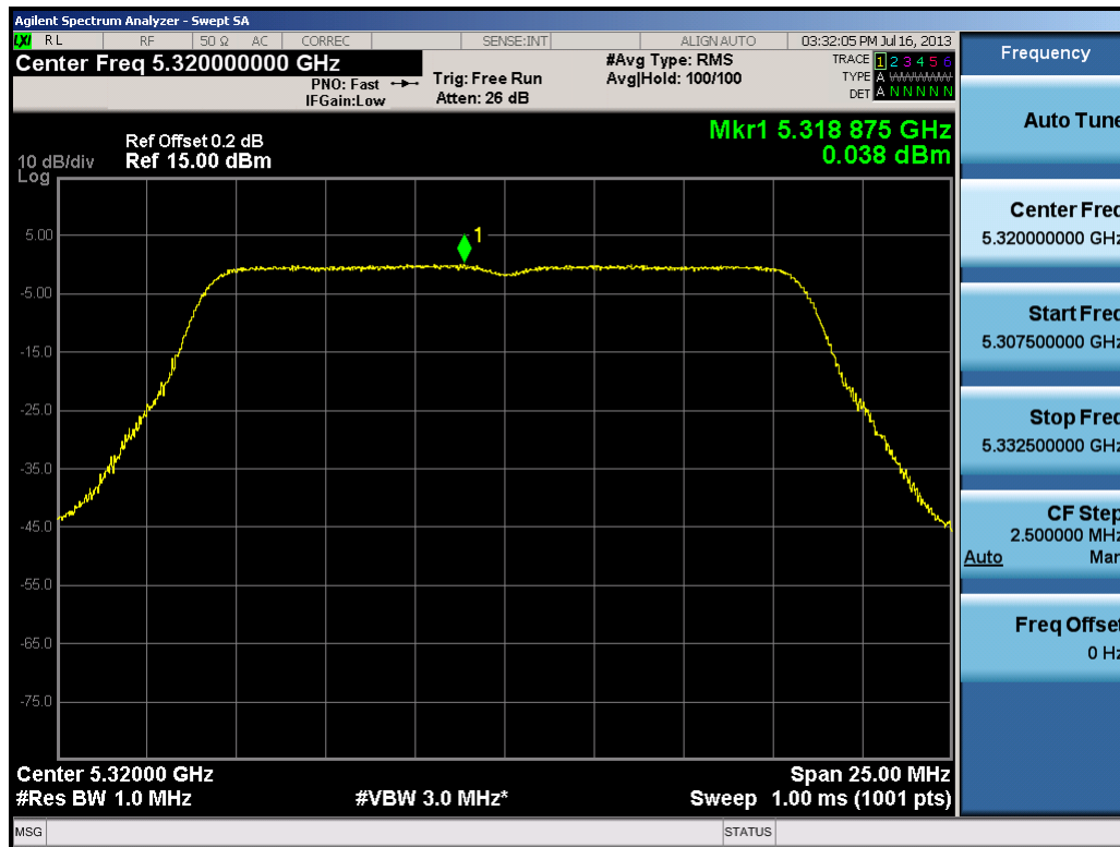
Plot 6-53. Peak Power Spectral Density Plot (802.11a (UNII Band 2) – Ch. 64)
