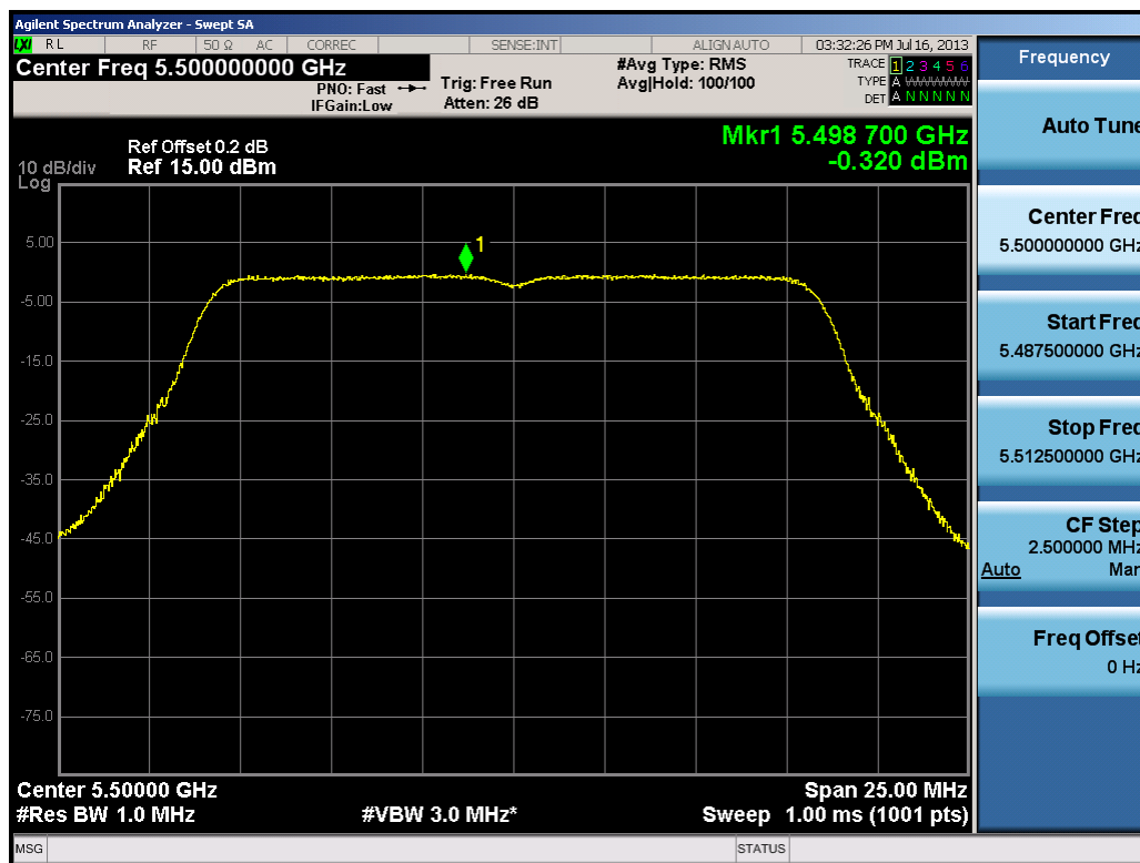
Plot 6-60. Peak Power Spectral Density Plot (802.11a (UNII Band 3) – Ch. 100)
