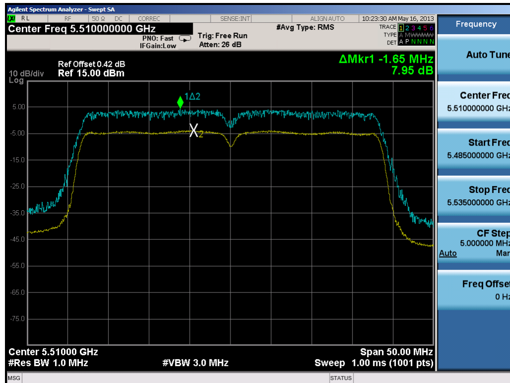
Plot 6-82. Peak Excursion Ratio Plot (40MHz BW 802.11n)
