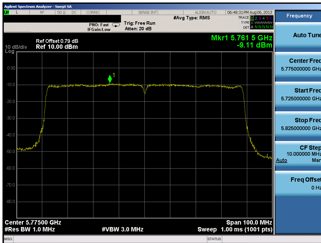
Plot 6-79. Peak Power Spectral Density Plot (80MHz BW 802.11ac (UNII Band 4) – Ch. 155)
