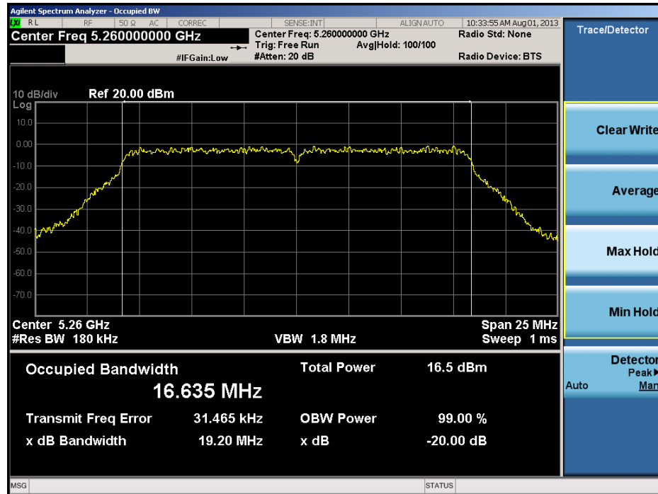
Plot 6-39. 20dB Bandwidth Plot (20MHz BW 802.11a (UNII Band 2) – Ch. 52)
