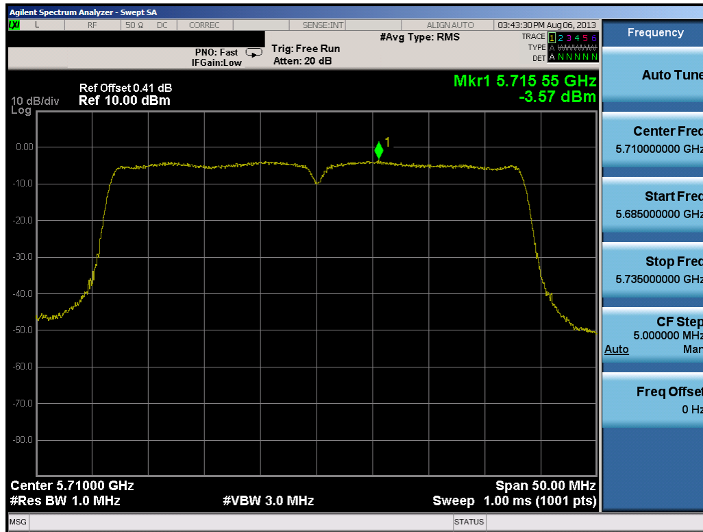
Plot 6-68. Peak Power Spectral Density Plot (40MHz BW 802.11n (UNII Band 3) – Ch. 142)
