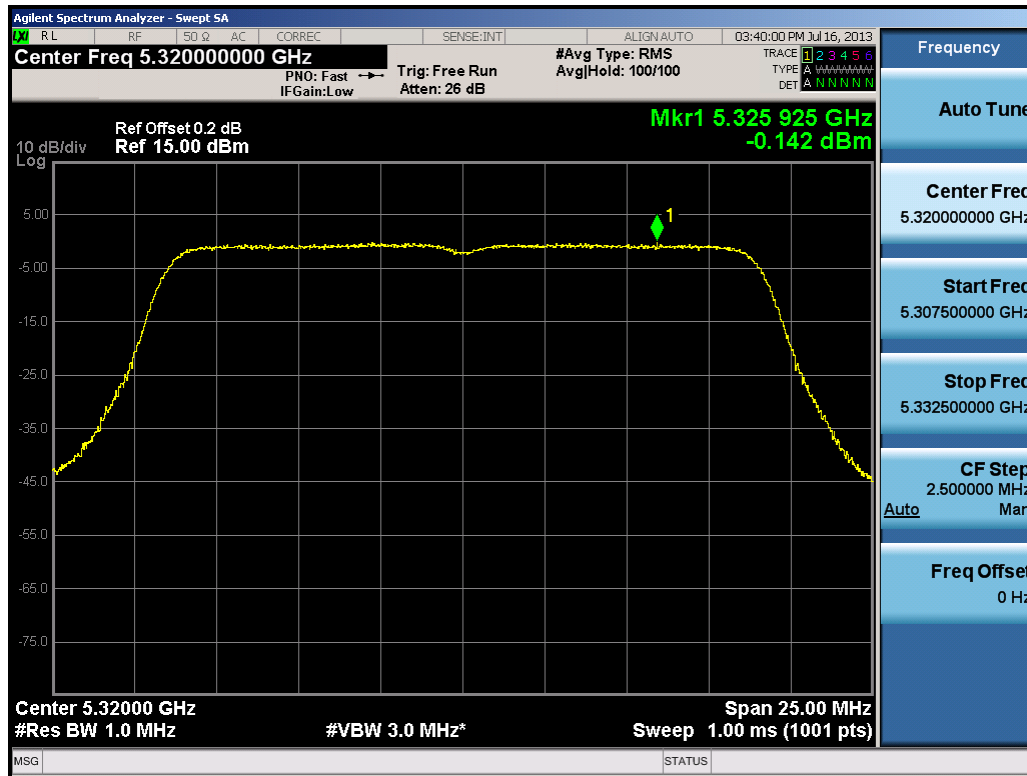
Plot 6-56. Peak Power Spectral Density Plot (20MHz BW 802.11n (UNII Band 2) – Ch. 64)
