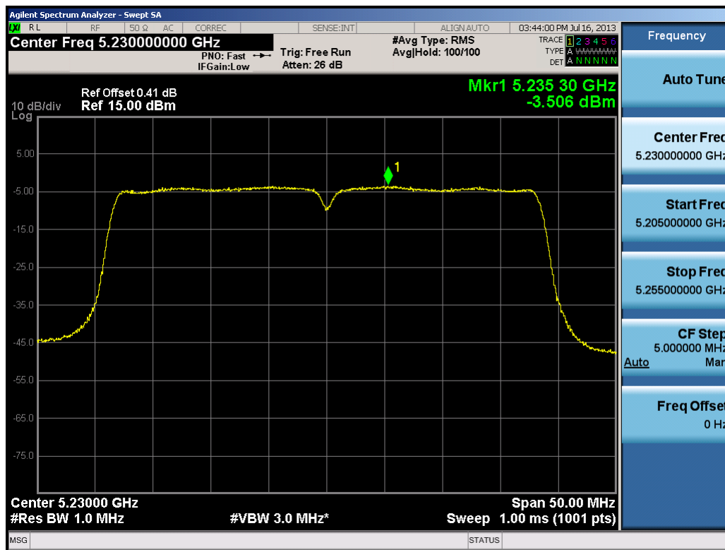
Plot 6-49. Peak Power Spectral Density Plot (40MHz BW 802.11n (UNII Band 1) – Ch. 46)
