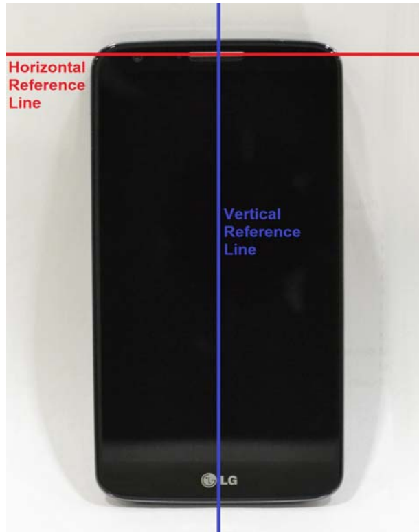
SAR Test Setup Photo 11 – DUT Reference Lines
