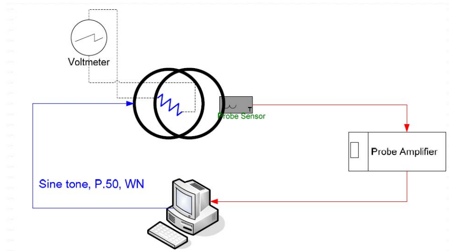
Figure 5-1 Validation Setup with Helmholtz Coil
