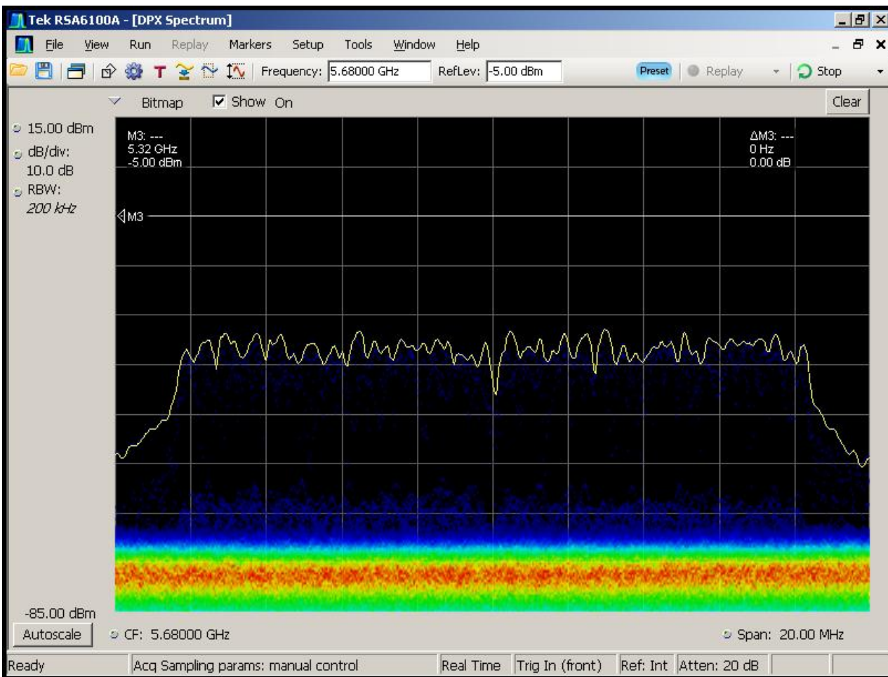
Figure 6-3. Real-Time Spectrum Display, WLAN Traffic (Streaming Video)
