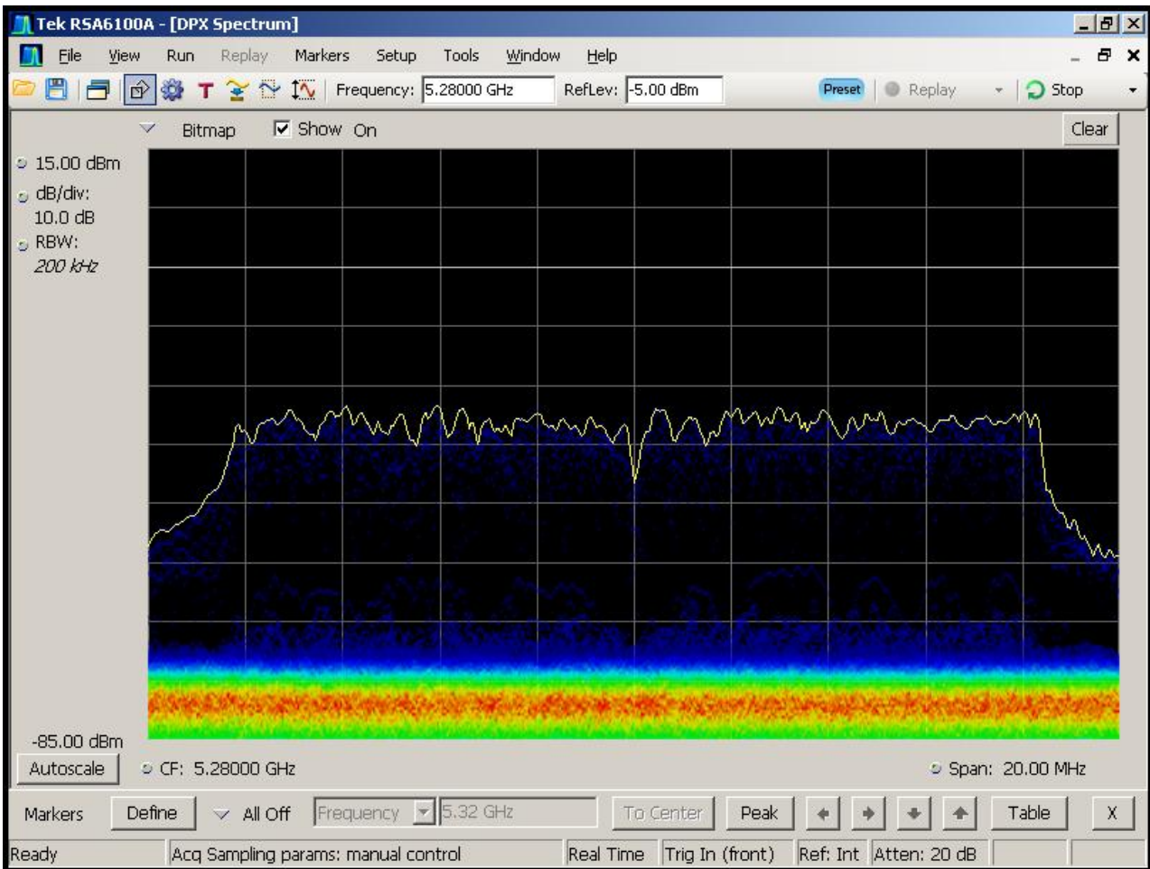
Figure 5-3. Real-Time Spectrum Display, WLAN Traffic (Streaming Video)
