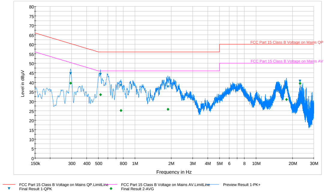
Plot 6-107. Line Conducted Plot with 802.11a UNII Band 4 (L1)
