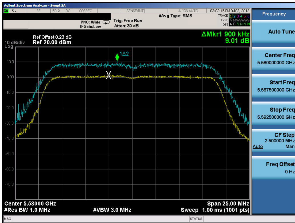
Plot 6-77. Peak Excursion Ratio Plot (20MHz BW 802.11n)
