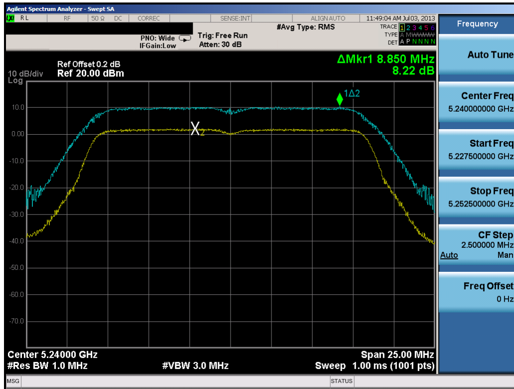
Plot 6-76. Peak Excursion Ratio Plot (802.11a)
