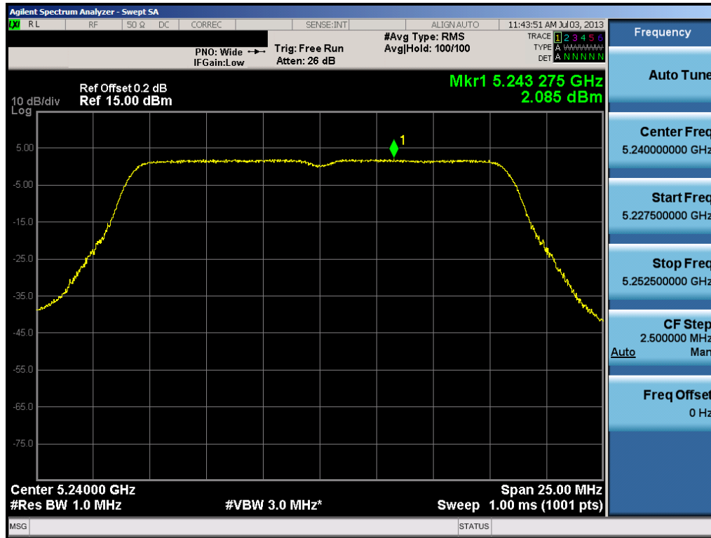
Plot 6-41. Peak Power Spectral Density Plot (802.11a (UNII Band 1) – Ch. 48)
