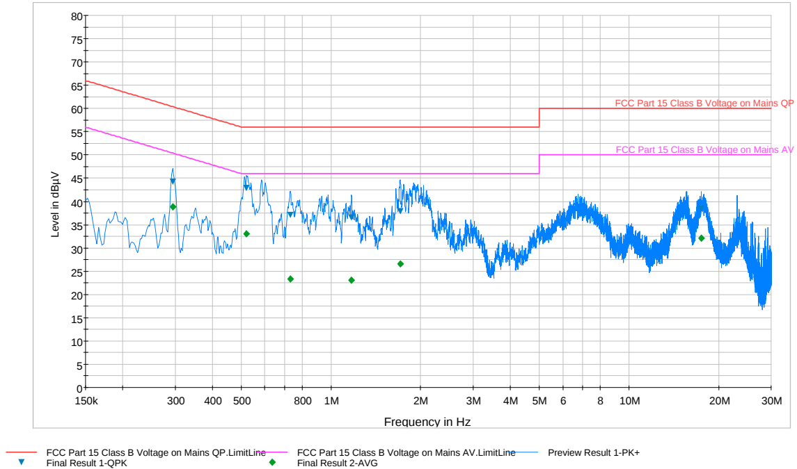
Plot 6-101. Line Conducted Plot with 802.11a UNII Band 1 (L1)
