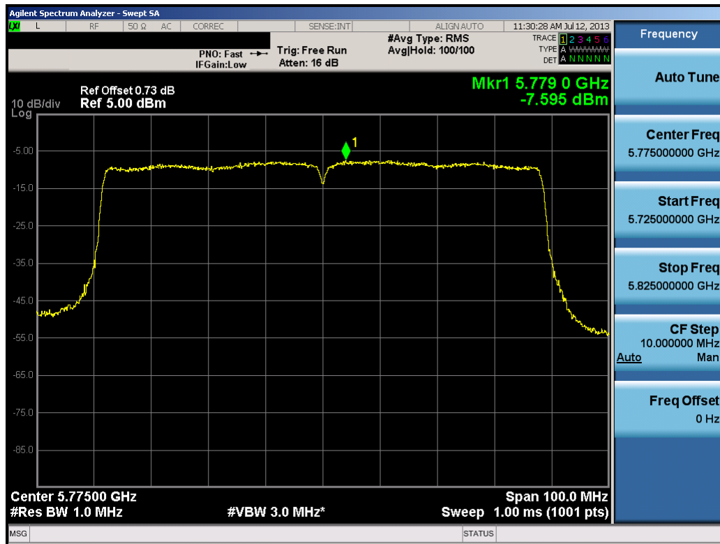
Plot 6-75. Peak Power Spectral Density Plot (80MHz BW 802.11ac (UNII Band 4) – Ch. 155)
