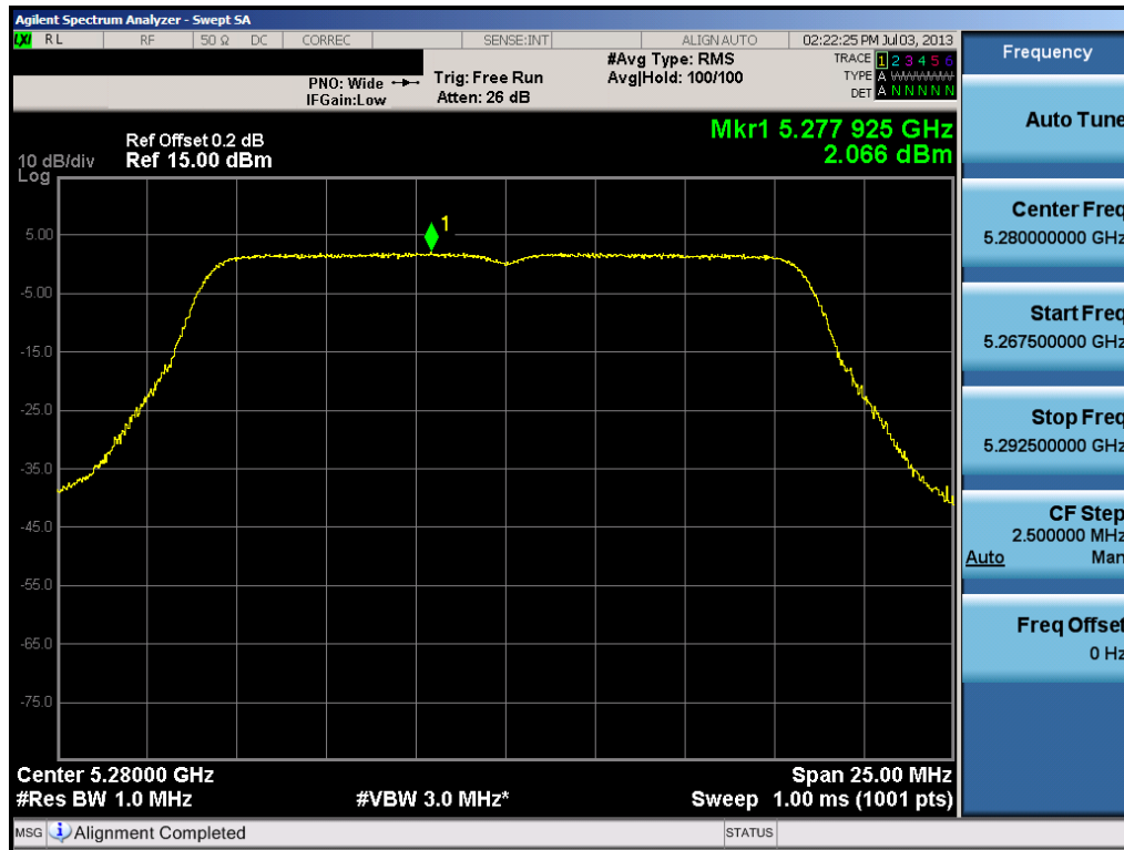
Plot 6-49. Peak Power Spectral Density Plot (802.11a (UNII Band 2) – Ch. 56)
