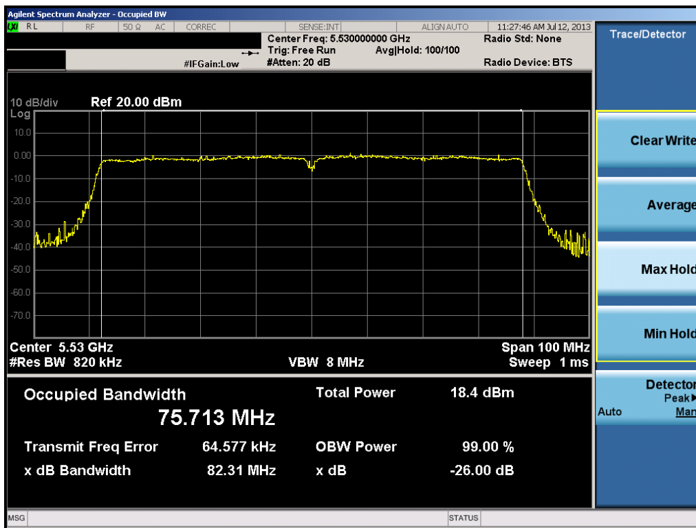
Plot 6-28. 26dB Bandwidth Plot (80MHz BW 802.11ac (UNII Band 3) – Ch. 106)
