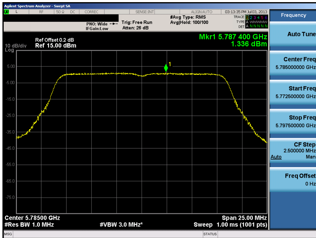
Plot 6-68. Peak Power Spectral Density Plot (20MHz BW 802.11a (UNII Band 4) – Ch. 157)
