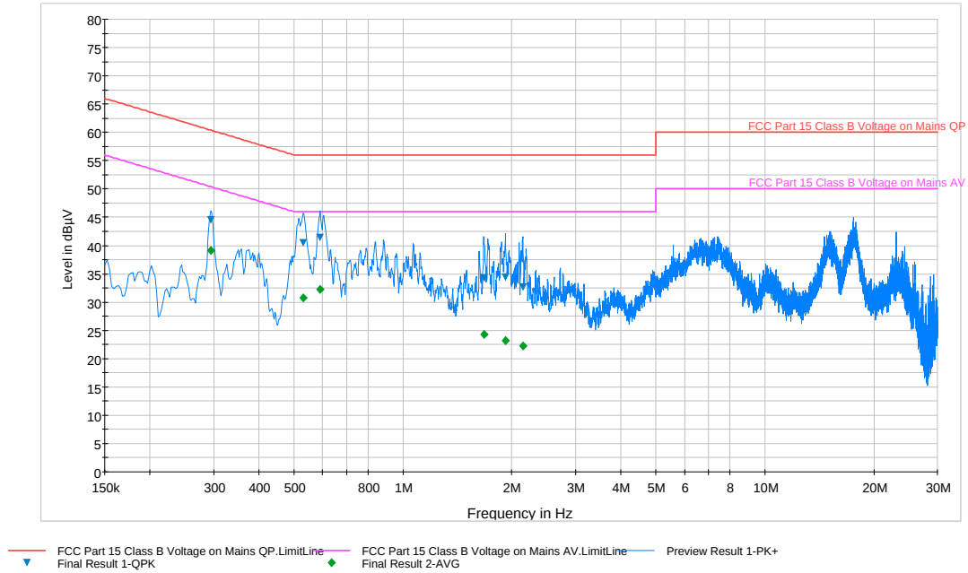
Plot 6-108. Line Conducted Plot with 802.11a UNII Band 4 (N)
