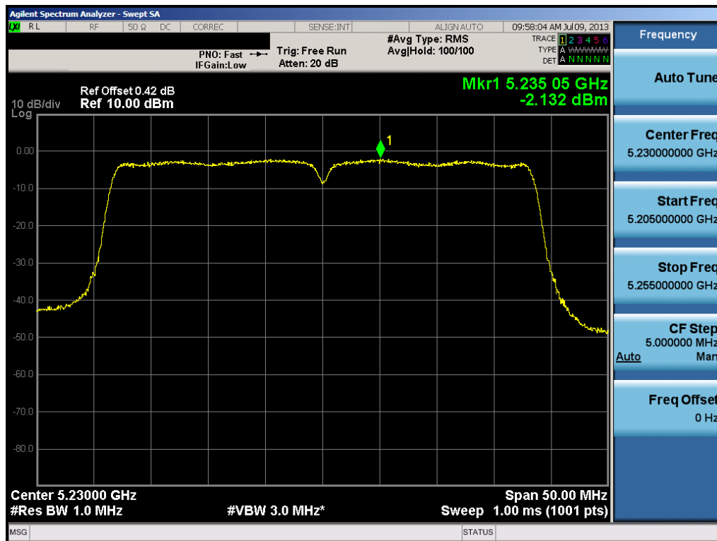
Plot 6-46. Peak Power Spectral Density Plot (40MHz BW 802.11n (UNII Band 1) – Ch. 46)
