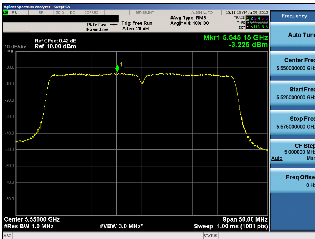
Plot 6-64. Peak Power Spectral Density Plot (40MHz BW 802.11n (UNII Band 3) – Ch. 110)
