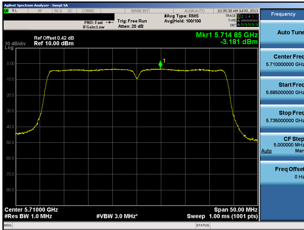
Plot 6-65. Peak Power Spectral Density Plot (40MHz BW 802.11n (UNII Band 3) – Ch. 142)
