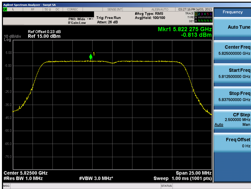
Plot 6-72. Peak Power Spectral Density Plot (20MHz BW 802.11n (UNII Band 4) – Ch. 165)
