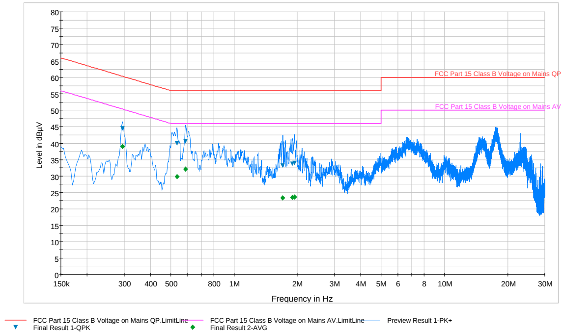
Plot 6-102. Line Conducted Plot with 802.11a UNII Band 1 (N)
