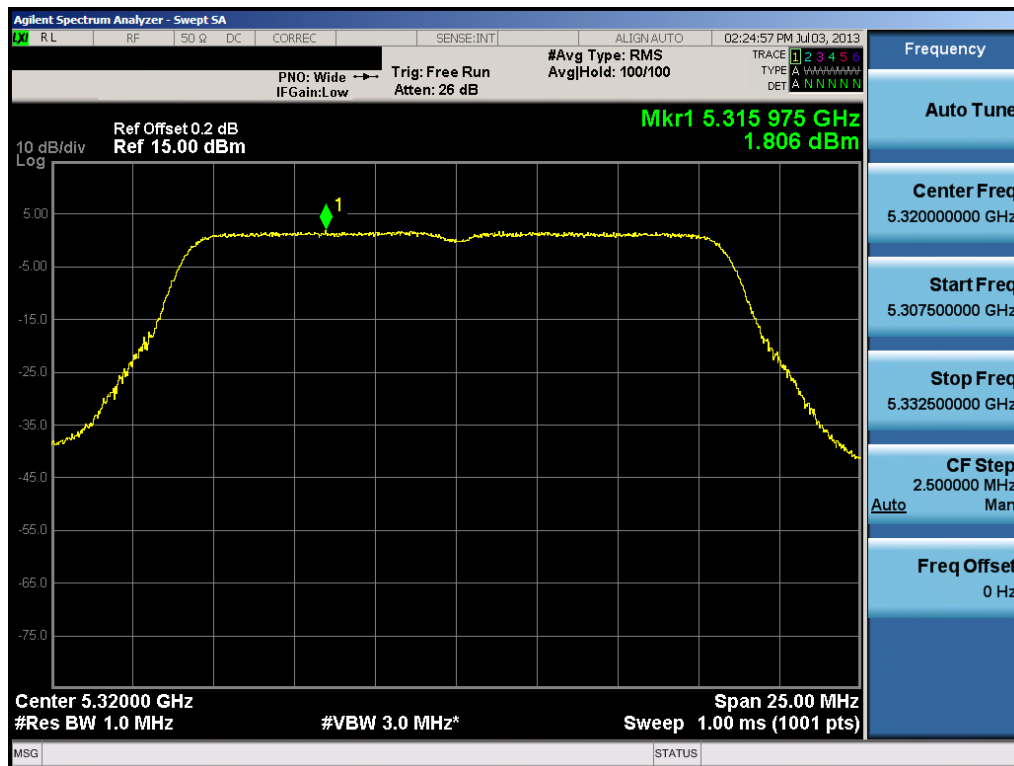
Plot 6-50. Peak Power Spectral Density Plot (802.11a (UNII Band 2) – Ch. 64)
