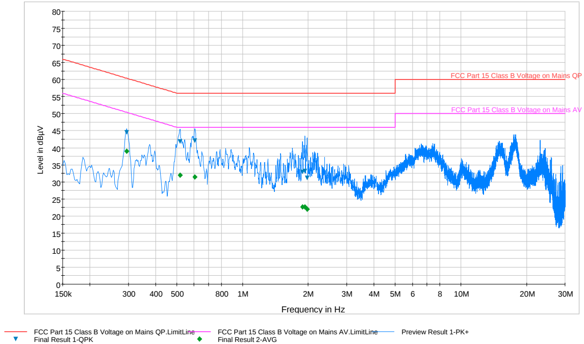
Plot 6-106. Line Conducted Plot with 802.11a UNII Band 3 (N)
