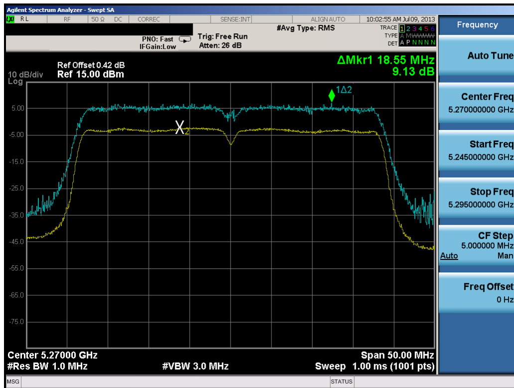
Plot 6-78. Peak Excursion Ratio Plot (40MHz BW 802.11n)
