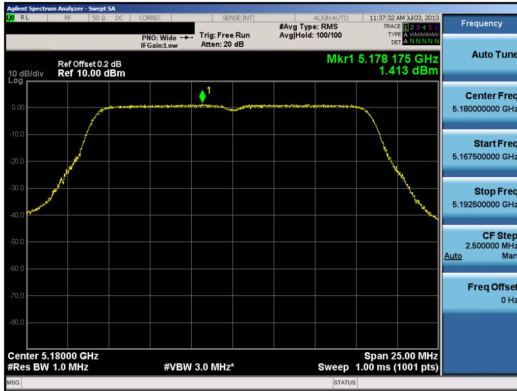
Plot 6-39. Peak Power Spectral Density Plot (802.11a (UNII Band 1) – Ch. 36)
