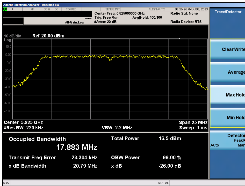
Plot 6-34. 26dB Bandwidth Plot (20MHz BW 802.11n (UNII Band 4) – Ch. 165)
