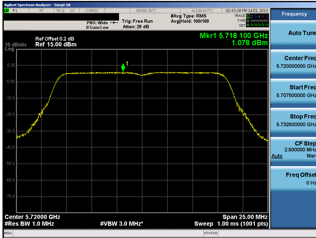
Plot 6-59. Peak Power Spectral Density Plot (802.11a (UNII Band 3) – Ch. 144)
