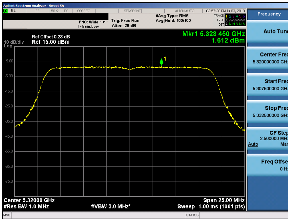
Plot 6-53. Peak Power Spectral Density Plot (20MHz BW 802.11n (UNII Band 2) – Ch. 64)
