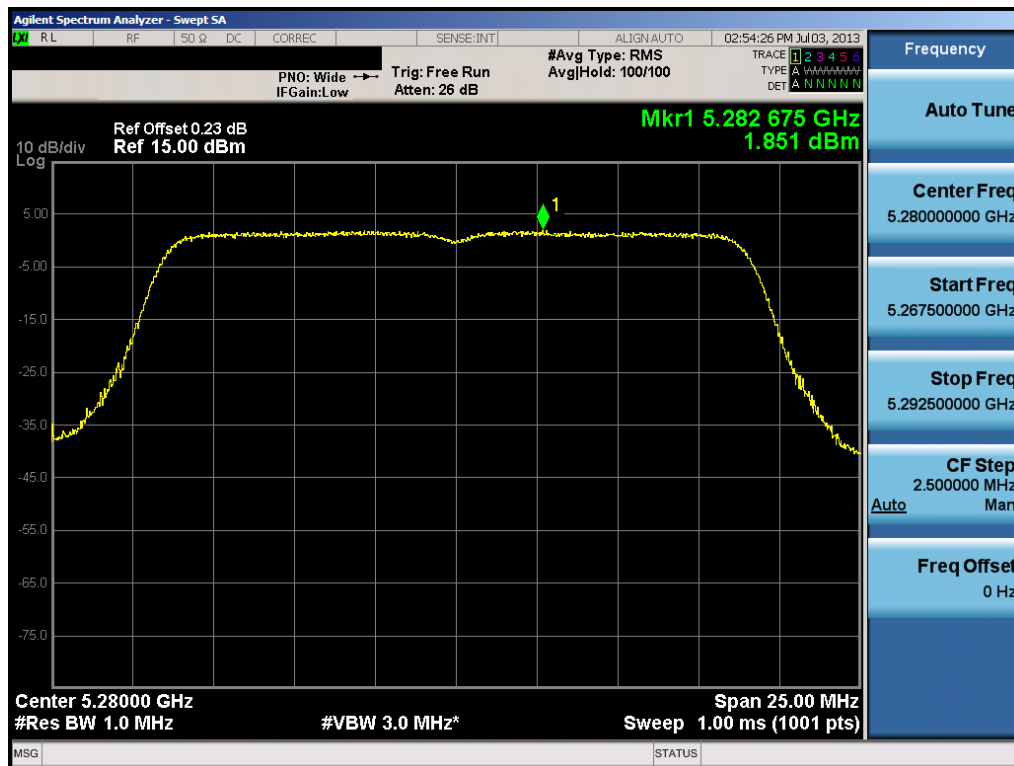
Plot 6-52. Peak Power Spectral Density Plot (20MHz BW 802.11n (UNII Band 2) – Ch. 56)
