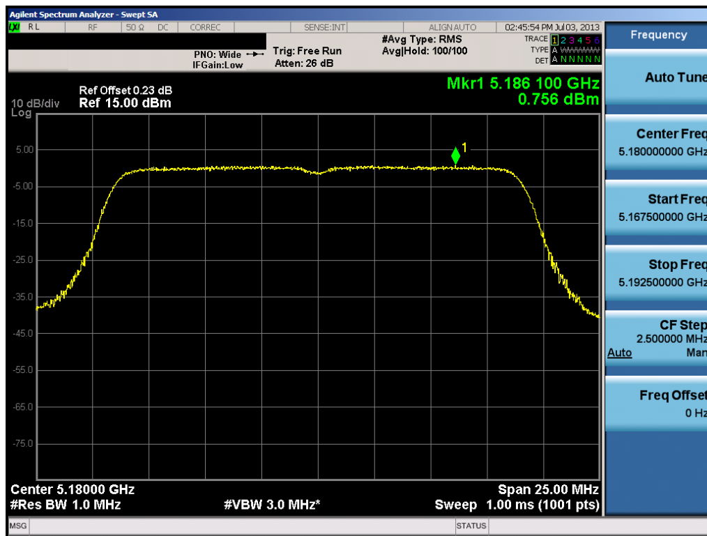
Plot 6-42. Peak Power Spectral Density Plot (20MHz BW 802.11n (UNII Band 1) – Ch. 36)
