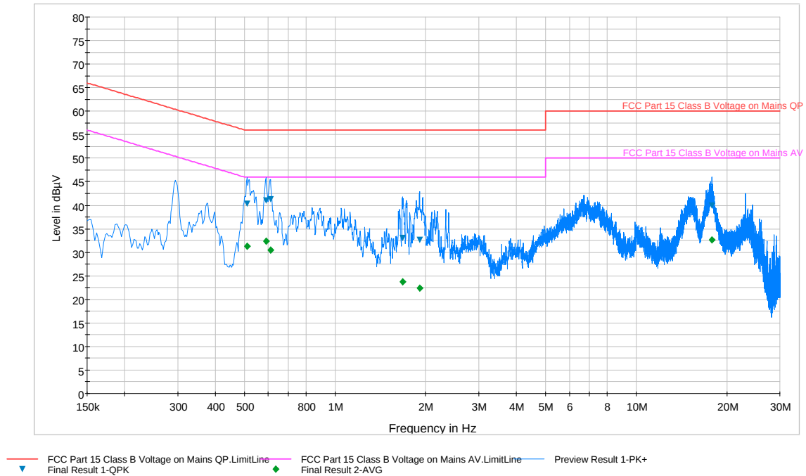
Plot 6-104. Line Conducted Plot with 802.11a UNII Band 2 (N)
