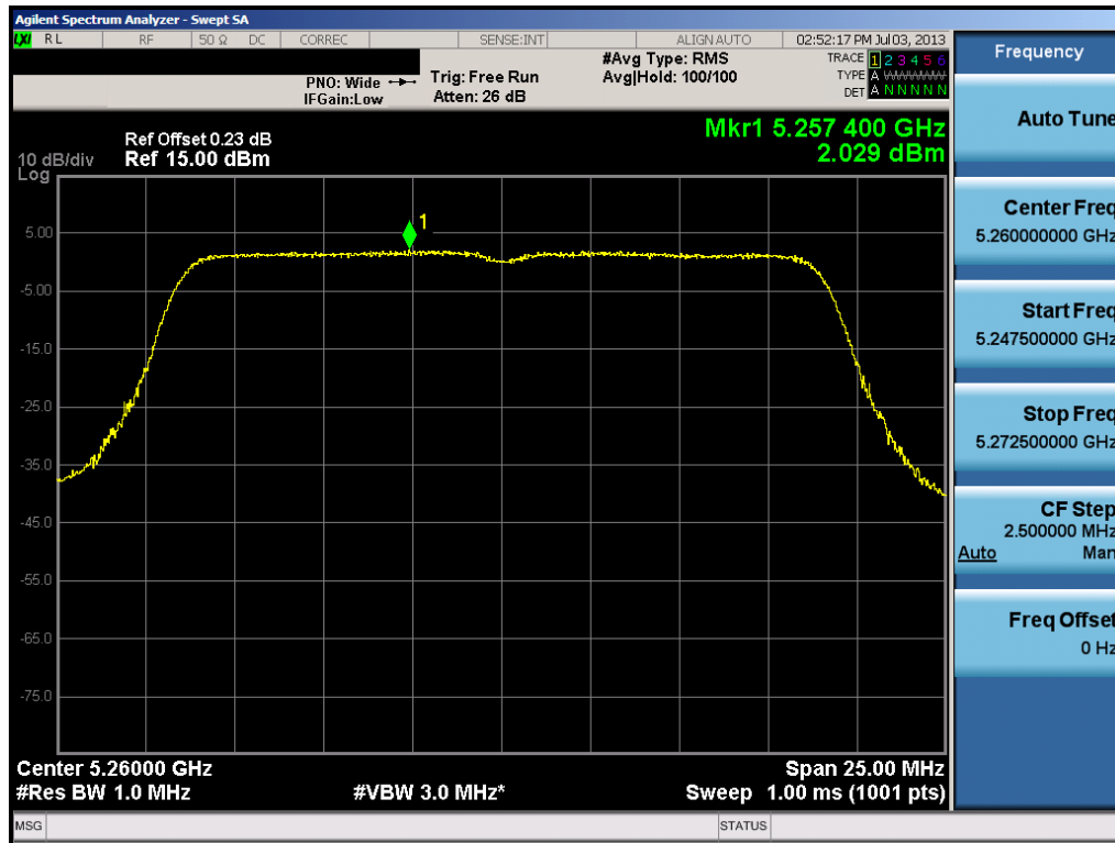
Plot 6-51. Peak Power Spectral Density Plot (20MHz BW 802.11n (UNII Band 2) – Ch. 52)
