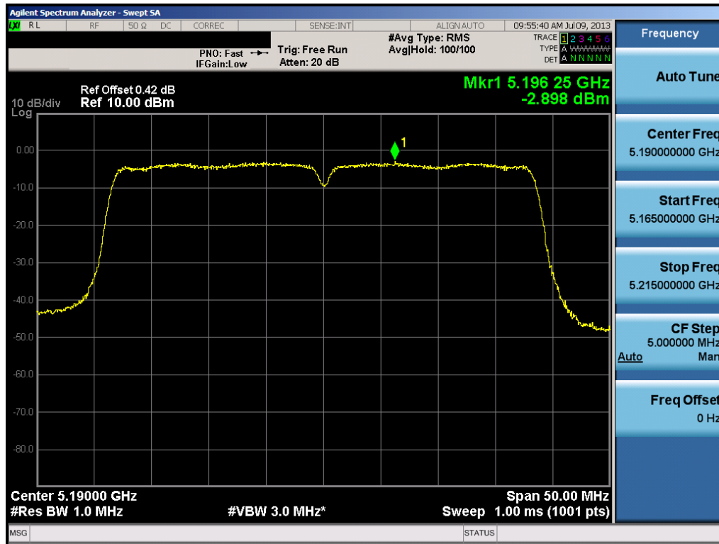
Plot 6-45. Peak Power Spectral Density Plot (40MHz BW 802.11n (UNII Band 1) – Ch. 38)
