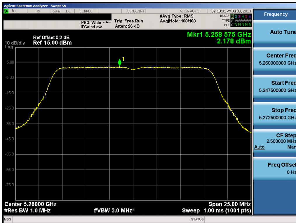
Plot 6-48. Peak Power Spectral Density Plot (802.11a (UNII Band 2) – Ch. 52)
