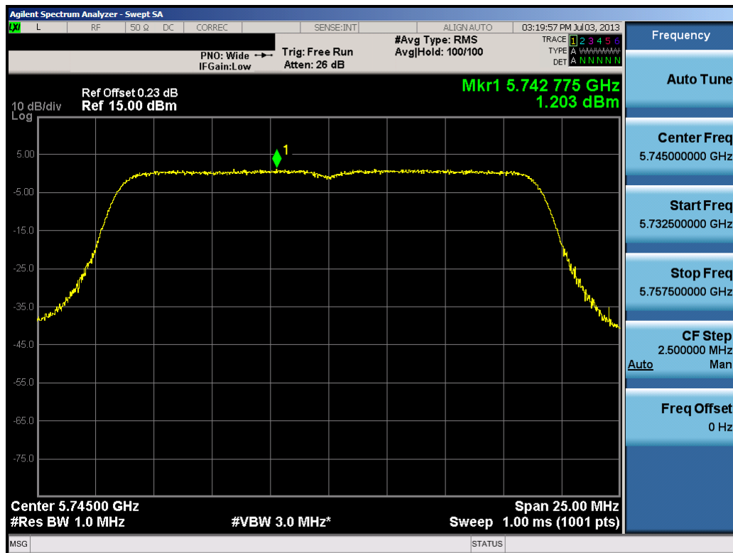
Plot 6-70. Peak Power Spectral Density Plot (20MHz BW 802.11n (UNII Band 4) – Ch. 149)
