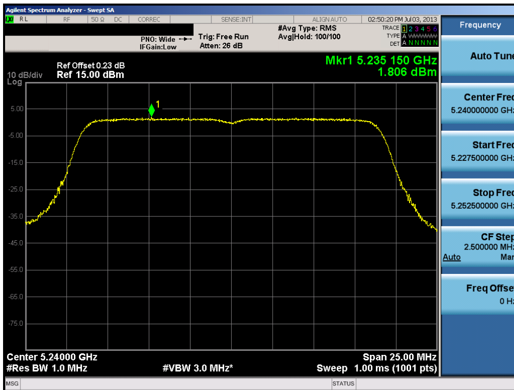
Plot 6-44. Peak Power Spectral Density Plot (20MHz BW 802.11n (UNII Band 1) – Ch. 48)
