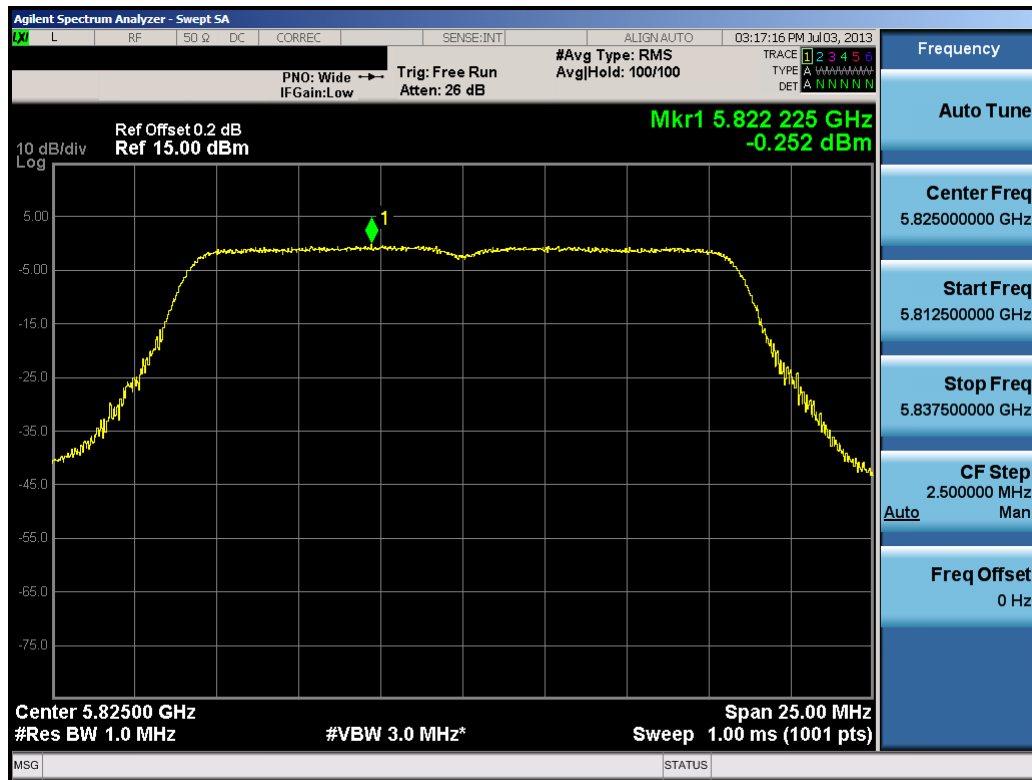
Plot 6-69. Peak Power Spectral Density Plot (20MHz BW 802.11a (UNII Band 4) – Ch. 165)
