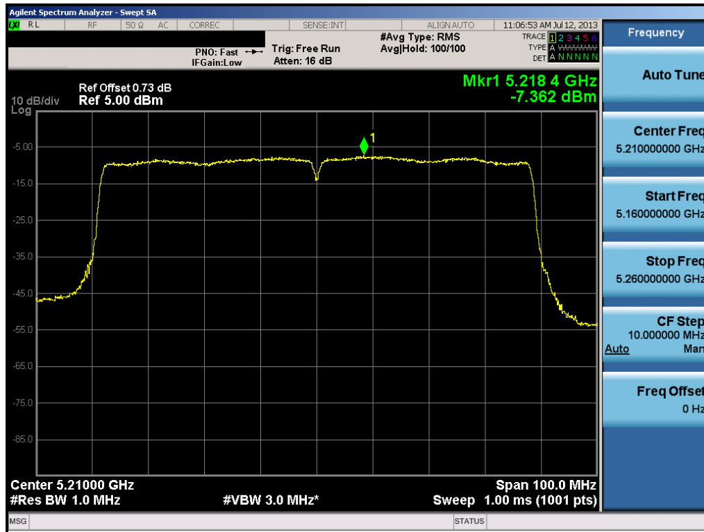
Plot 6-47. Peak Power Spectral Density Plot (80MHz BW 802.11ac (UNII Band 1) – Ch. 42)
