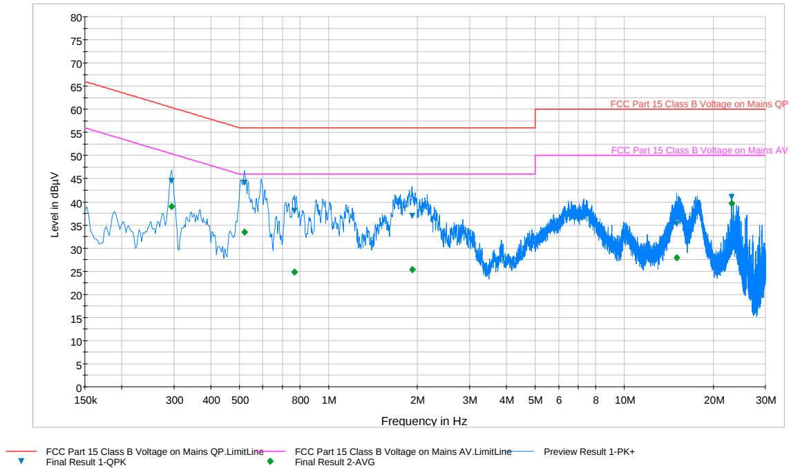
Plot 6-105. Line Conducted Plot with 802.11a UNII Band 3 (L1)
