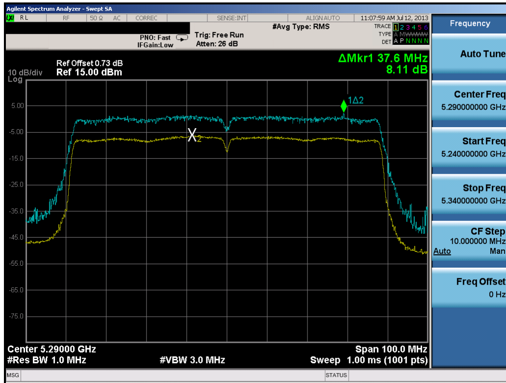
Plot 6-79. Peak Excursion Ratio Plot (80MHz BW 802.11ac)
