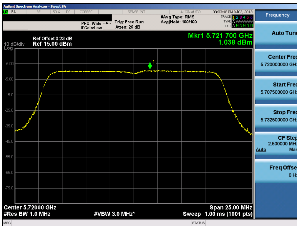
Plot 6-62. Peak Power Spectral Density Plot (20MHz BW 802.11n (UNII Band 3) – Ch. 144)
