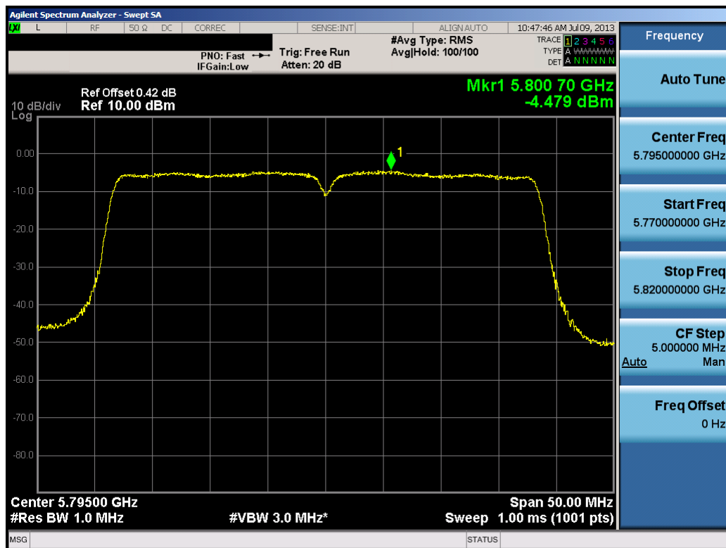
Plot 6-74. Peak Power Spectral Density Plot (40MHz BW 802.11n (UNII Band 4) – Ch. 159)
