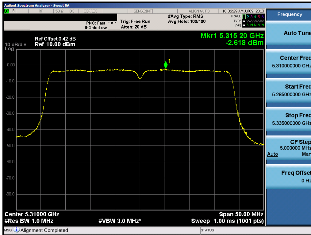
Plot 6-55. Peak Power Spectral Density Plot (40MHz BW 802.11n (UNII Band 2) – Ch. 62)
