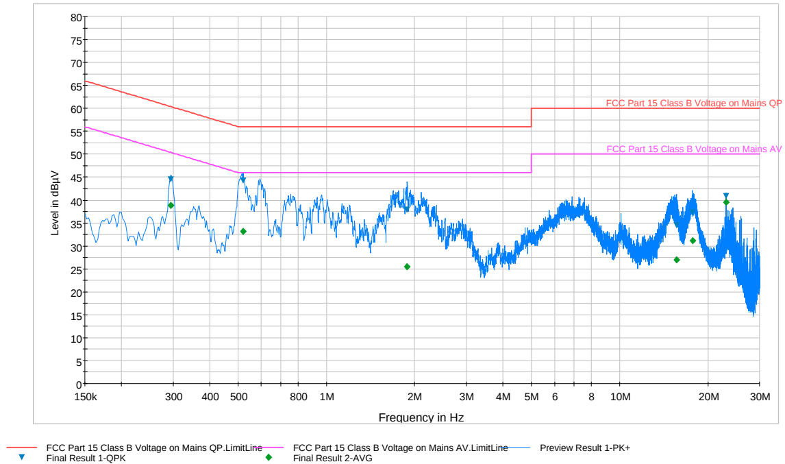
Plot 6-103. Line Conducted Plot with 802.11a UNII Band 2 (L1)
