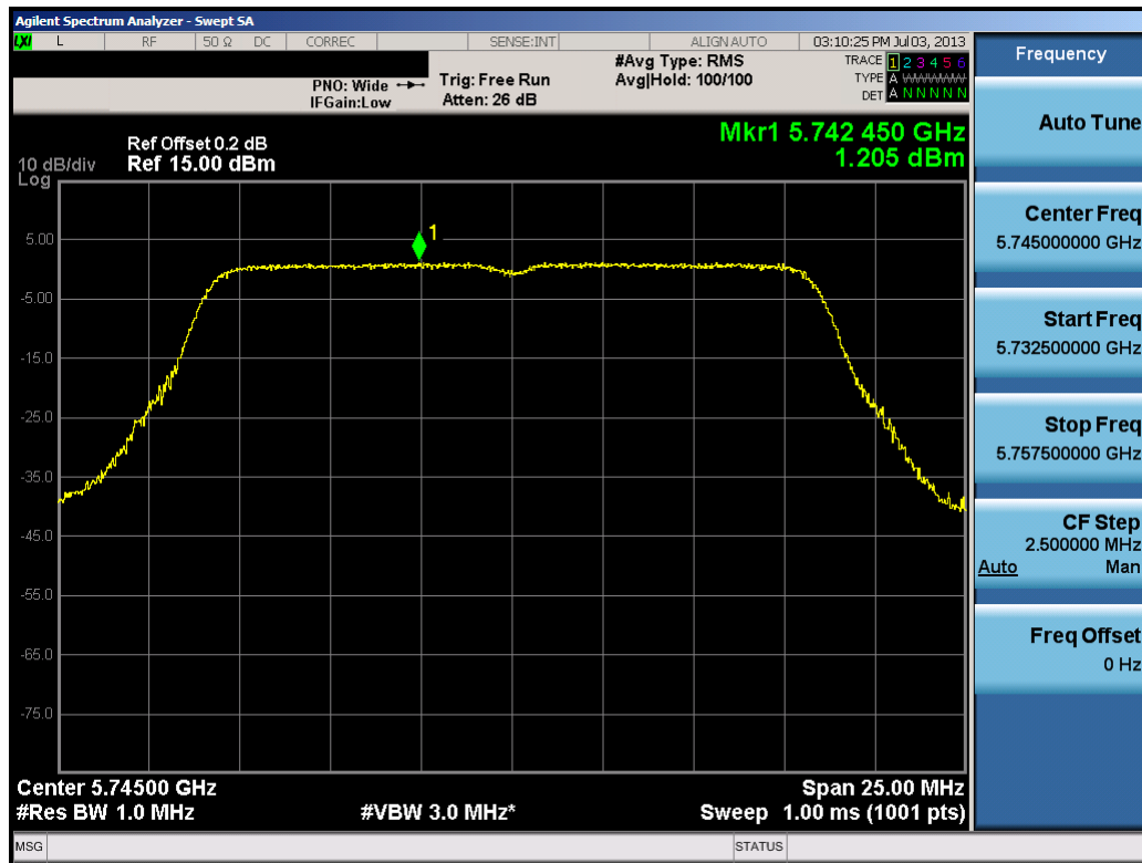
Plot 6-67. Peak Power Spectral Density Plot (20MHz BW 802.11a (UNII Band 4) – Ch. 149)
