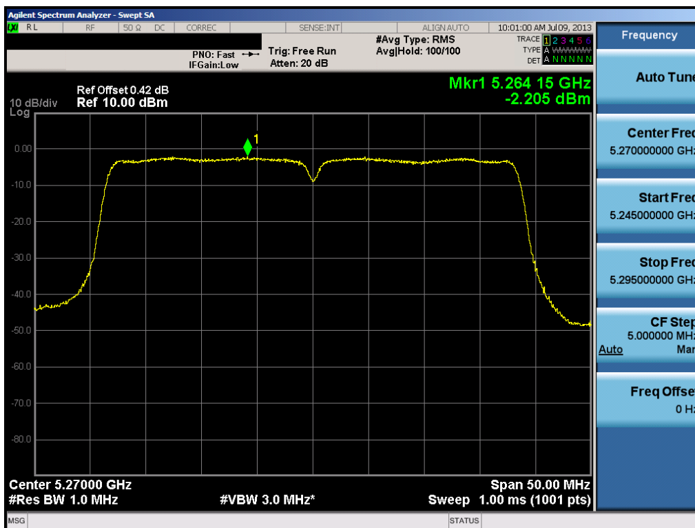
Plot 6-54. Peak Power Spectral Density Plot (40MHz BW 802.11n (UNII Band 2) – Ch. 54)
