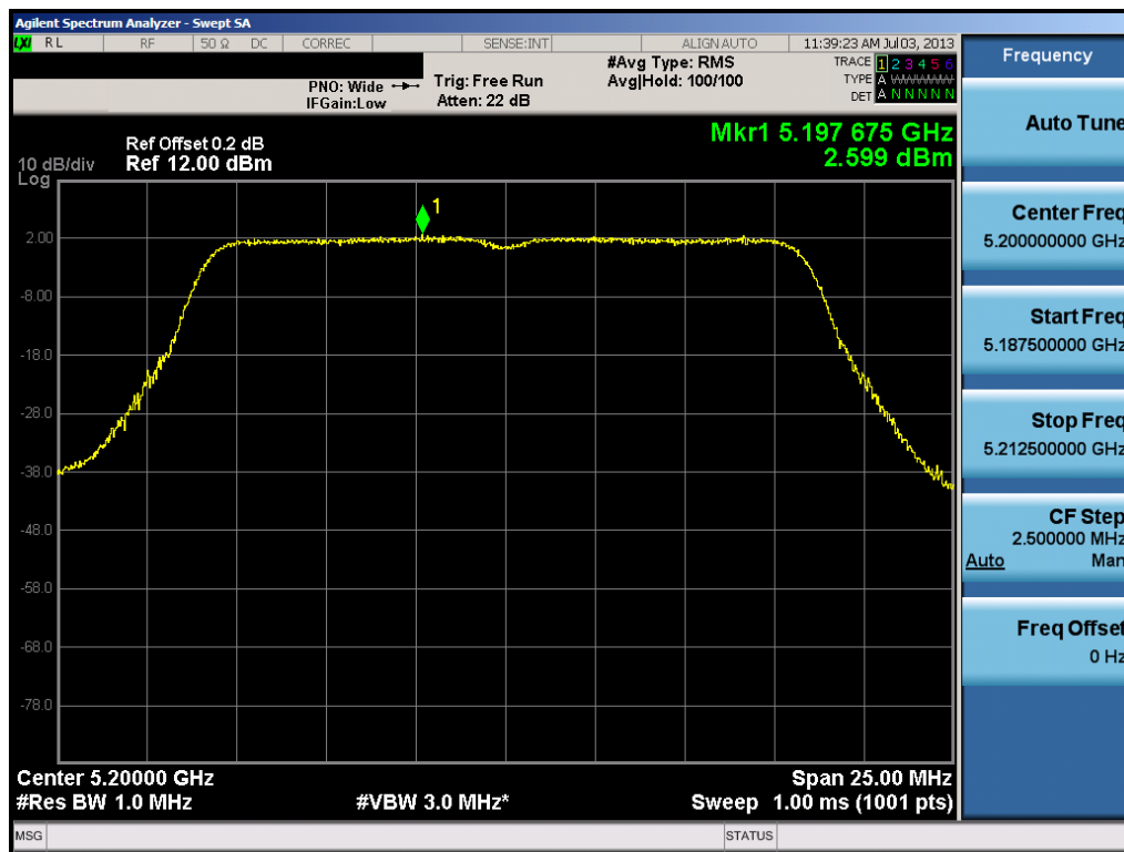
Plot 6-40. Peak Power Spectral Density Plot (802.11a (UNII Band 1) – Ch. 40)
