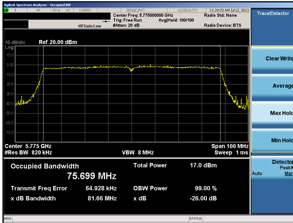
Plot 6-37. 26dB Bandwidth Plot (80MHz BW 802.11ac (UNII Band 4) – Ch. 155)
