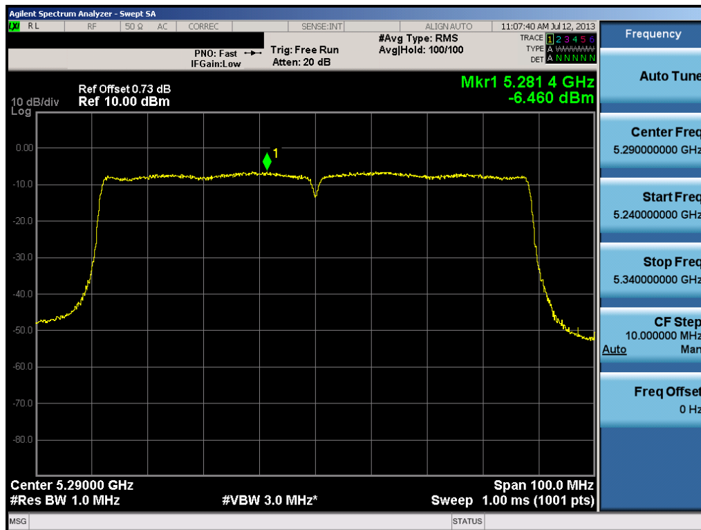
Plot 6-56. Peak Power Spectral Density Plot (80MHz BW 802.11ac (UNII Band 2) – Ch. 58)
