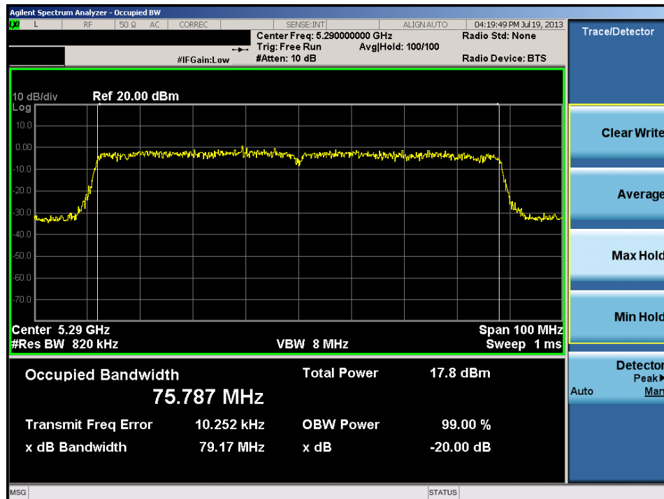
Plot 6-38. 20dB Bandwidth Plot (80MHz BW 802.11n (UNII Band 2) – Ch. 58)
