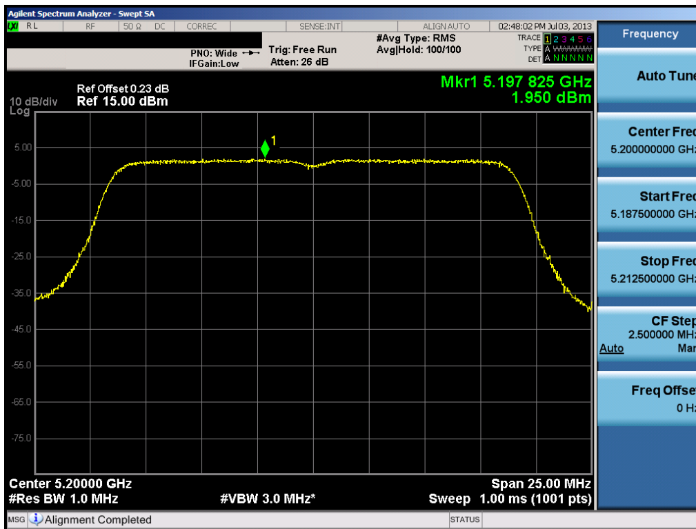
Plot 6-43. Peak Power Spectral Density Plot (20MHz BW 802.11n (UNII Band 1) – Ch. 40)
