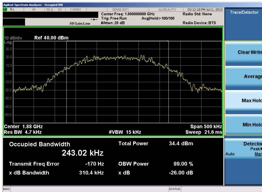
Plot 6-4. Occupied Bandwidth Plot (EDGE1900 Mode – Ch. 661)
