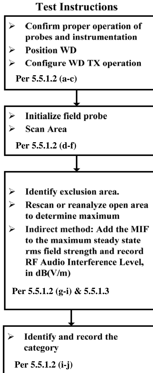
Figure 6-1 RF Emissions Flow Chart
