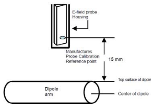
Figure 7-1 Separation Distance from Dipole to Field Probe
