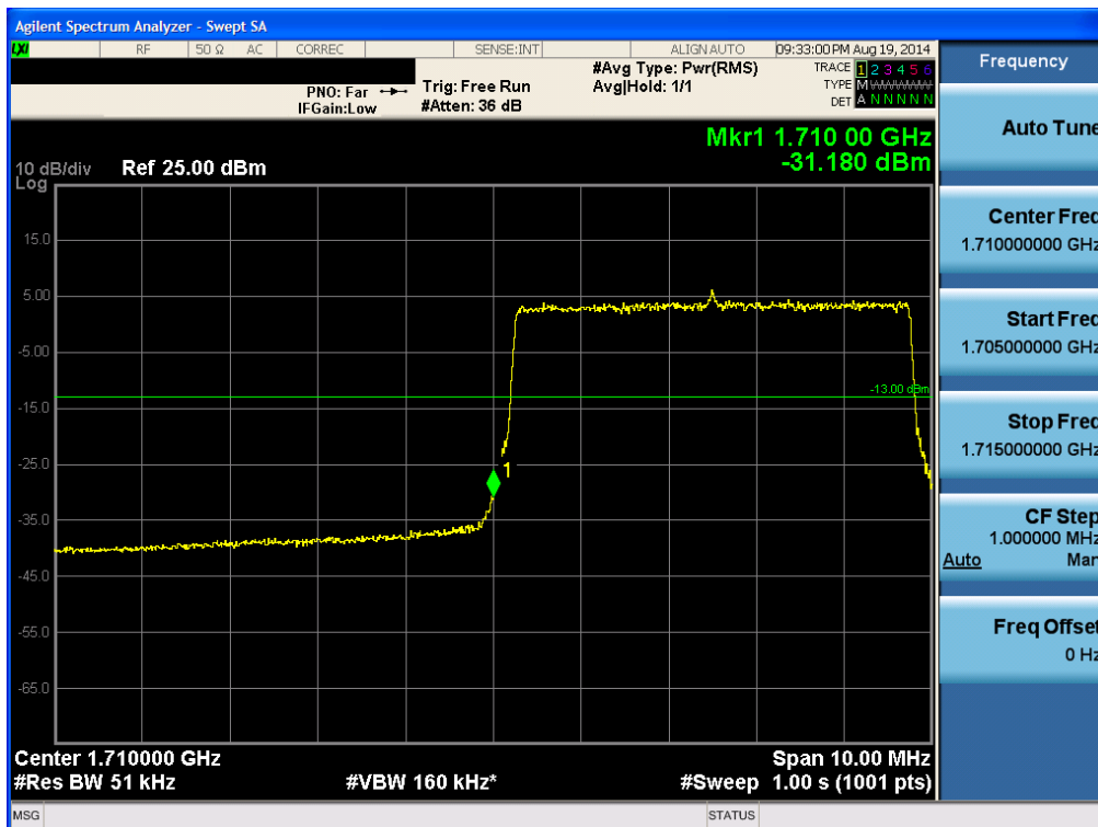
BAND 4. Lower Band Edge Plot (5M BW Ch.19975 QPSK RB 25) -2
