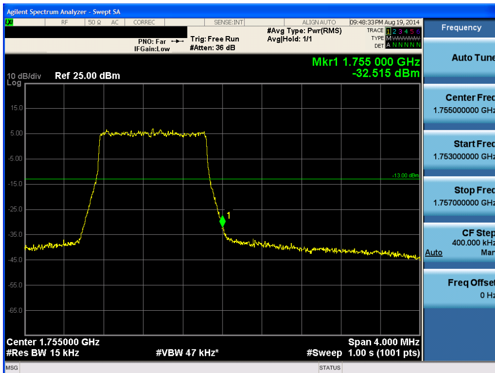
BAND 4. Upper Band Edge Plot (1.4M BW Ch.20393 QPSK RB 6) -2
