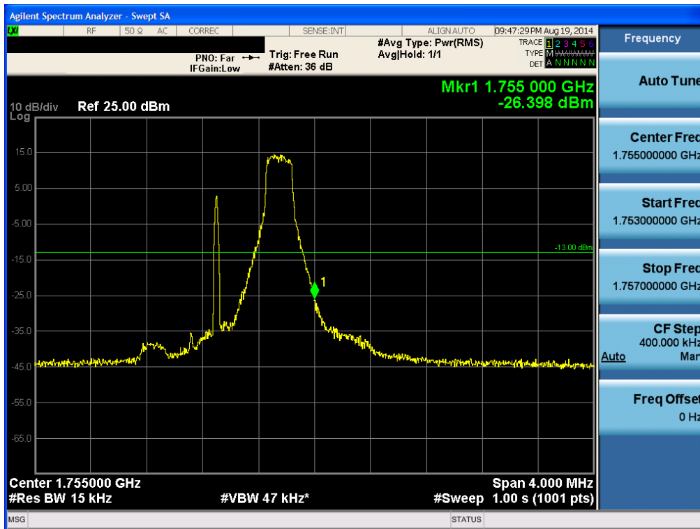
BAND 4. Upper Band Edge Plot (1.4M BW Ch.20393 QPSK RB 1, Offset 5) -1
