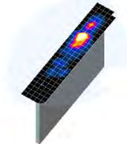
Figure 5.1 Sample SAR Area Scan
