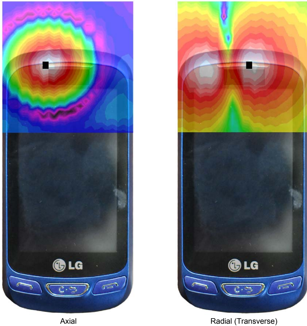
Figure 13-3 T-Coil Scan Overlay Magnetic Field Distributions
