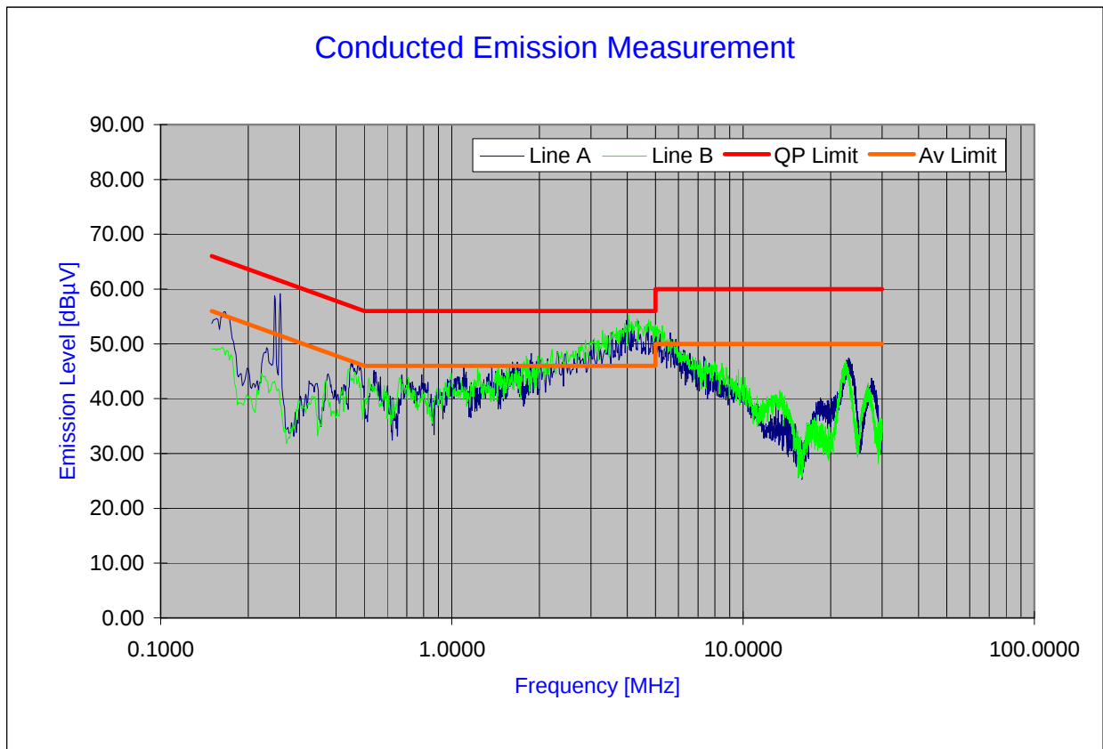
Plot 6-22. Line Conducted Plot with Bluetooth
