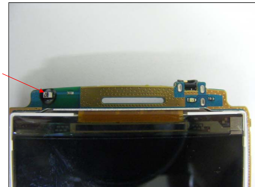
Bluetooth Antenna
