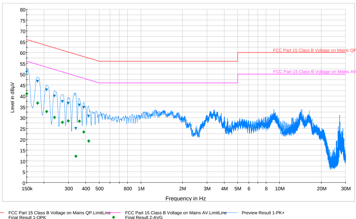
Plot 6-31. Line Conducted Plot with 802.11b (L1)
