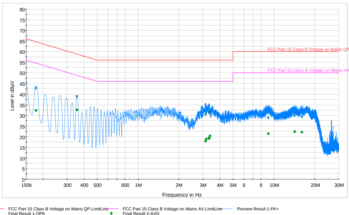
Plot 6-32. Line Conducted Plot with 802.11b (N)
