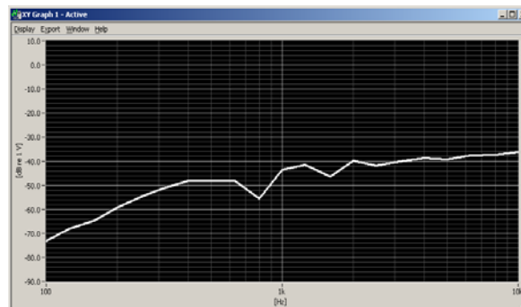
Figure 6-2 Worst-case ABM2 Plot for WD
