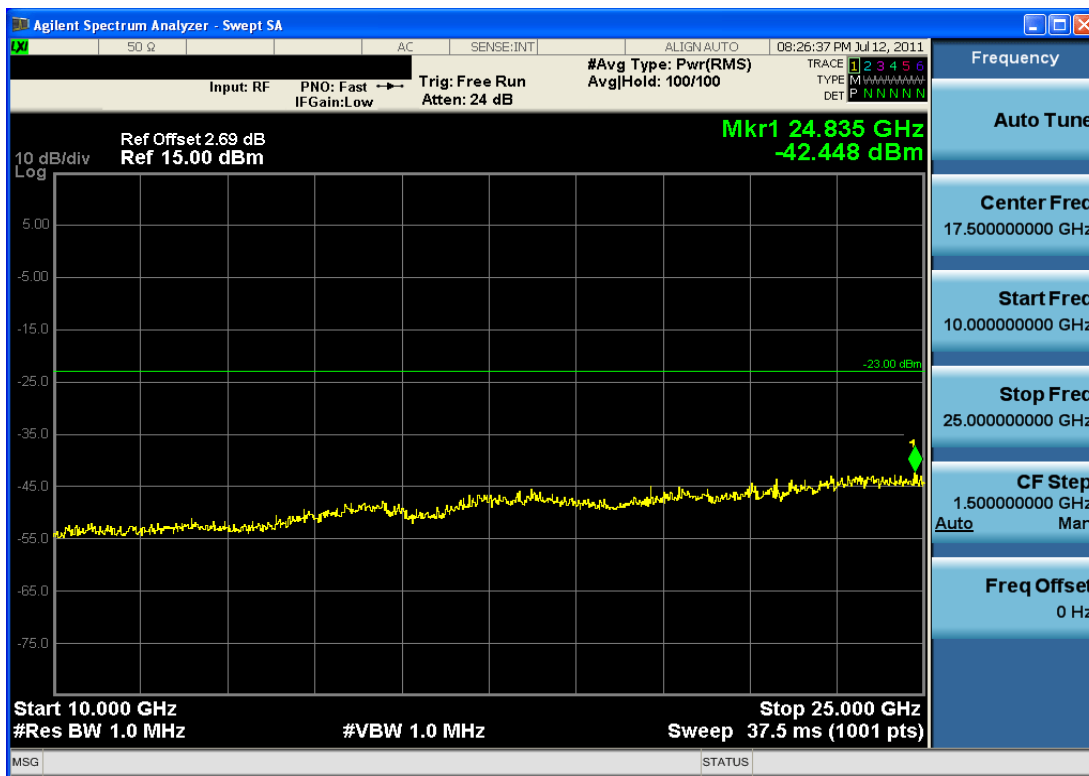
Plot 6-19. Conducted Spurious Plot (Bluetooth, 3Mbps – Ch. 0)
