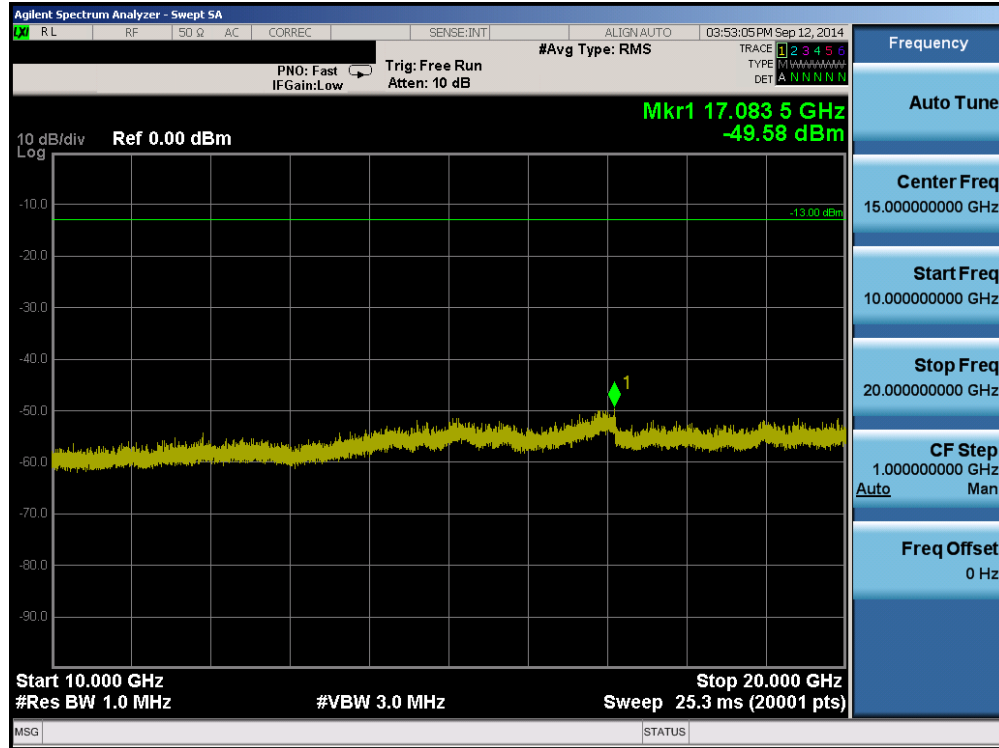
Plot 6-22. Conducted Spurious Plot (AWS WCDMA Mode – Ch. 1412)
