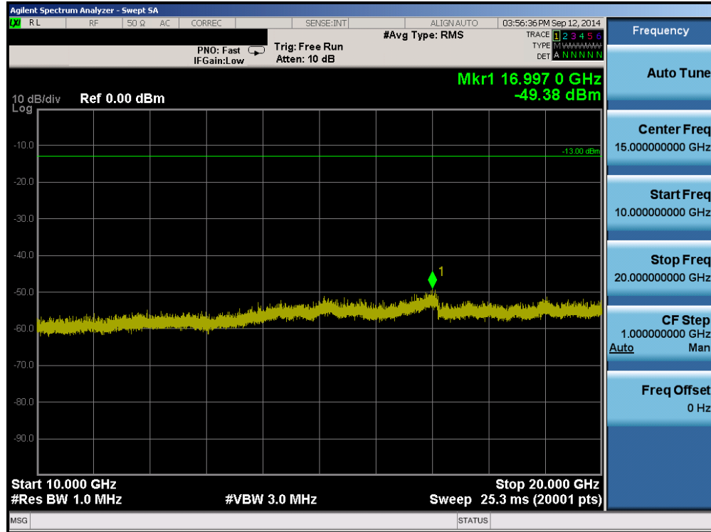
Plot 6-20. Conducted Spurious Plot (AWS WCDMA Mode – Ch. 1312)
