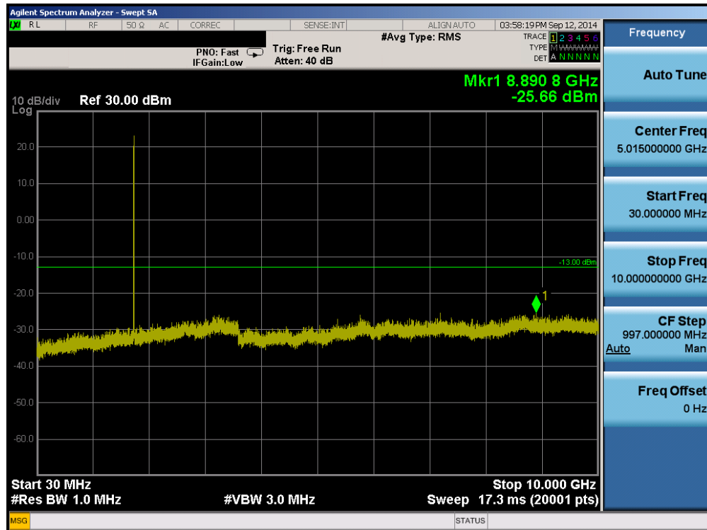
Plot 6-23. Conducted Spurious Plot (AWS WCDMA Mode – Ch. 1862)
