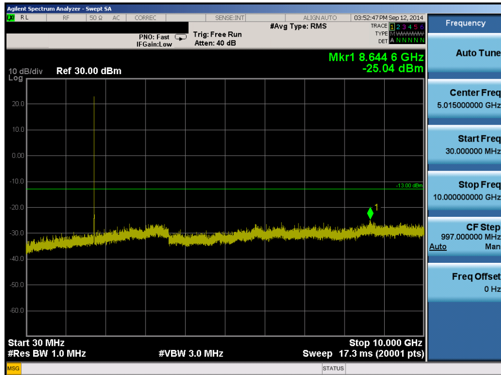
Plot 6-21. Conducted Spurious Plot (AWS WCDMA Mode – Ch. 1412)
