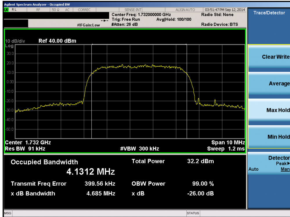
Plot 6-3. Occupied Bandwidth Plot (AWS WCDMA Mode – Ch. 1412)
