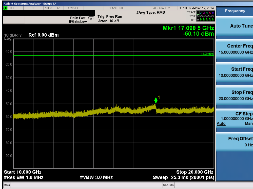
Plot 6-24. Conducted Spurious Plot (AWS WCDMA Mode – Ch. 1862)
