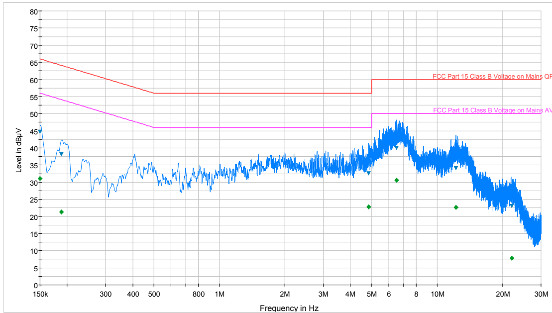
Plot 6-44. Line-Conducted Test Plot (L1)
