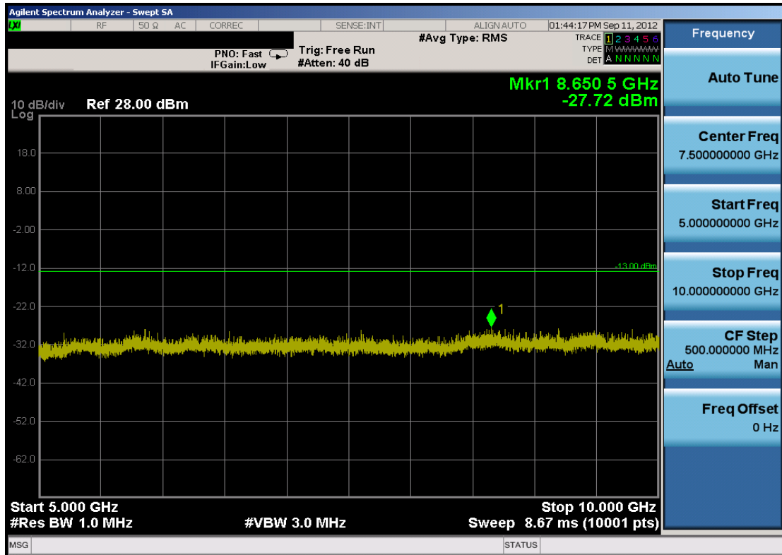
Plot 7-3. Conducted Spurious Plot (Cellular GSM Mode – Ch. 128)
