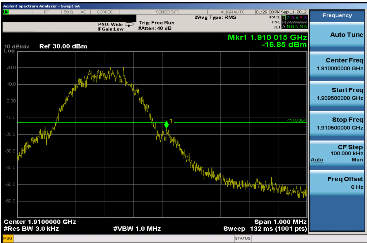
Plot 7-22. Band Edge Plot (PCS GSM Mode – Ch. 810)
