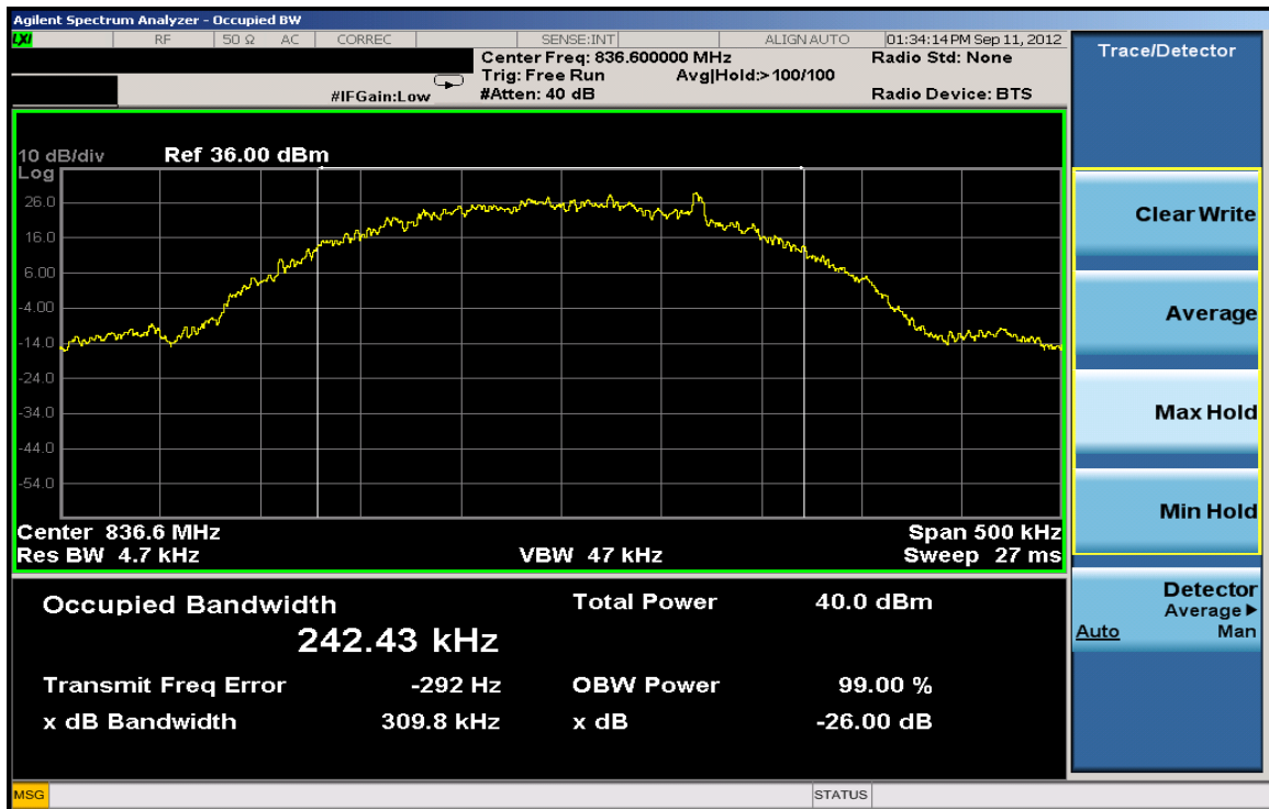
Plot 7-8. Occupied Bandwidth Plot (Cellular GSM Mode – Ch. 190)
