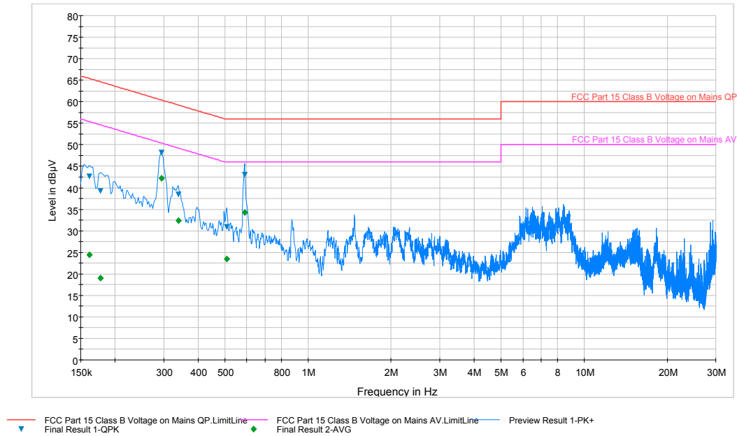
Plot 6-28. Line Conducted Plot with 802.11b (N)
