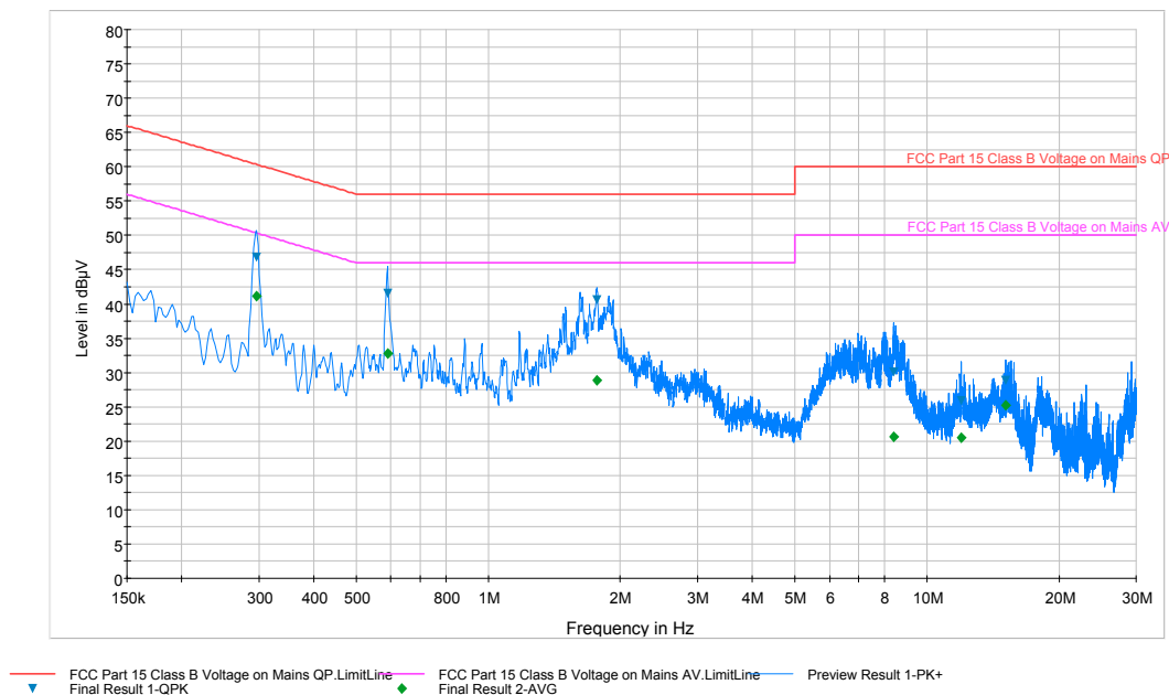
Plot 6-27. Line Conducted Plot with 802.11b (L1)
