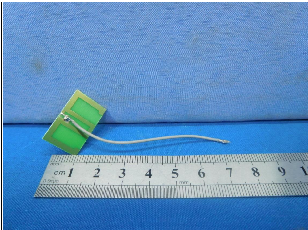
Antenna Model: 290-10434 (2.4GHz, Chain 0)
