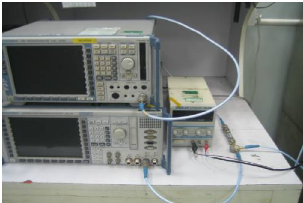
FREQUENCY STABILITY V.S. VOLTAGE MEASUREMENT Test Setup
