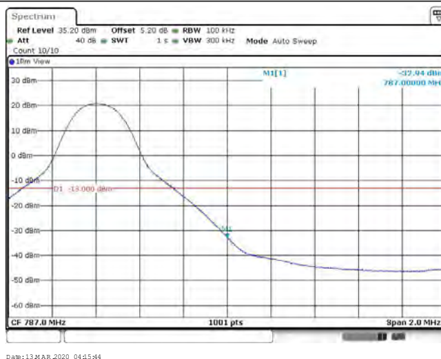
Band13_10MHz_QPSK_23230_Right_50RB#0
