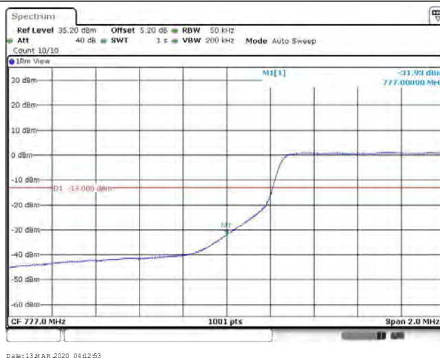
Band13_5MHz_16QAM_23255_1RB#24
