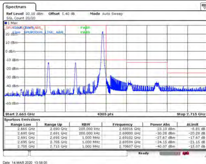
Band41_15MHz_16QAM_41515_75RB#0
