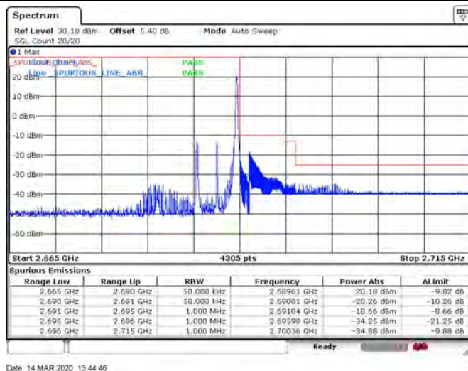
Band41_5MHz_QPSK_41565_25RB#0
