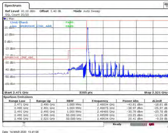
Band41_5MHz_16QAM_39675_25RB#0
