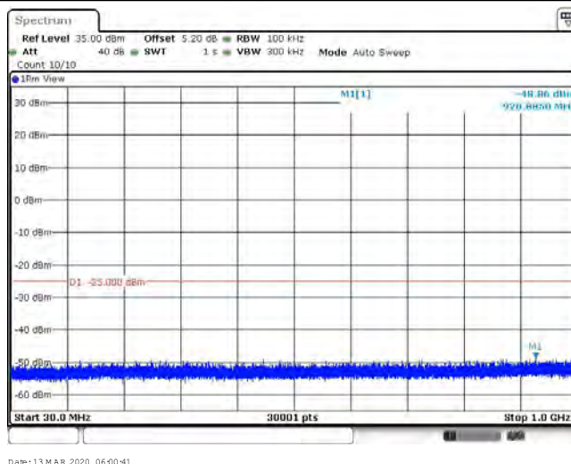
Band41_20MHz_16QAM_41490_1RB#0
