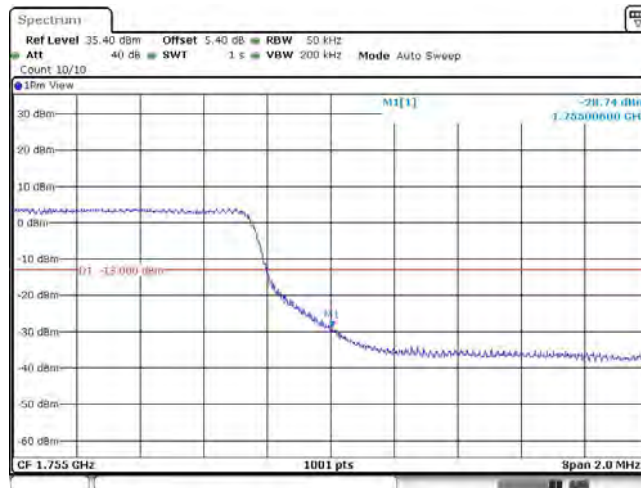
Band4_5MHz_QPSK_20375_25RB#0
