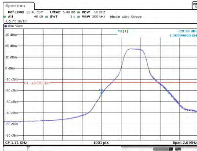
Band4_5MHz_16QAM_19975_25RB#0
