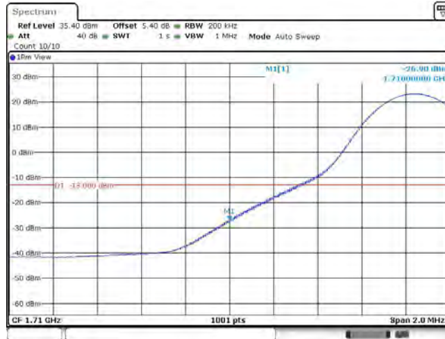
Band4_15MHz_QPSK_20025_75RB#0
