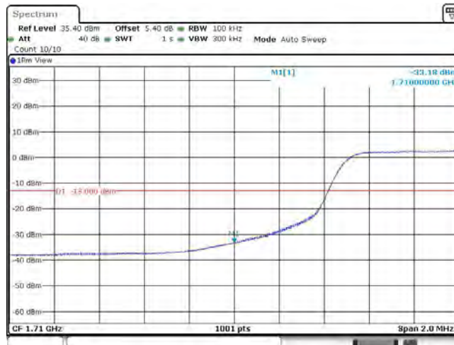
Band4_10MHz_16QAM_2000_50RB#0
