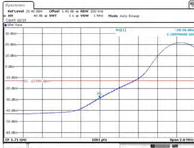
Band4_15MHz_16QAM_2025_75RB#0
