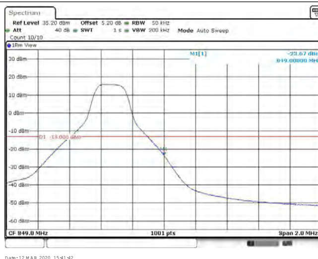
Band5 5MHz 16QAM 20625 25RB#0
