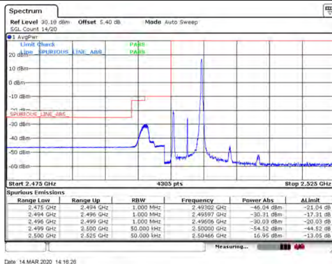
Band7_5MHz_16QAM_20775_25RB#0
