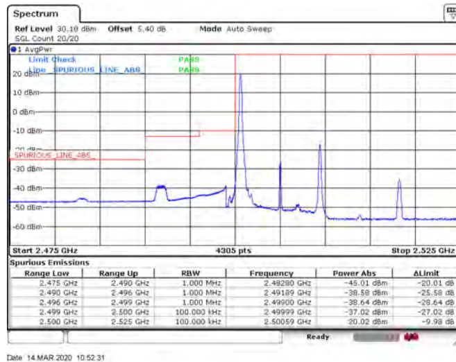
Band7_10MHz_QPSK_20800_50RB#0
