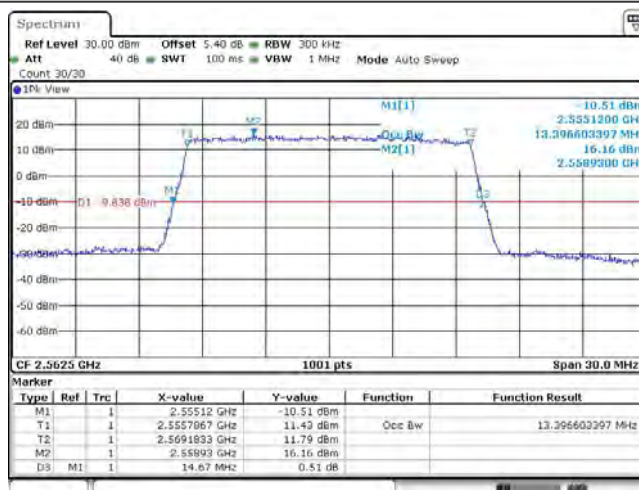
Band7 15MHz 16QAM 21375 75RB#0
