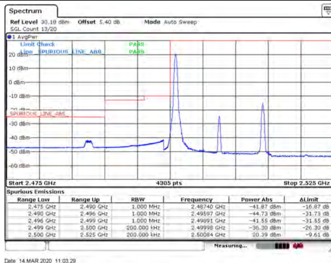
Band7_15MHz_16QAM_20825_75RB#0
