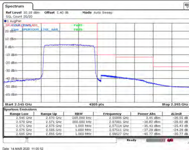
Band7_15MHz_QPSK_21375_75RB#0
