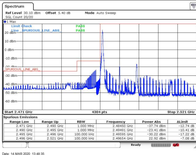
Band41_10MHz_16QAM_39700_50RB#0
