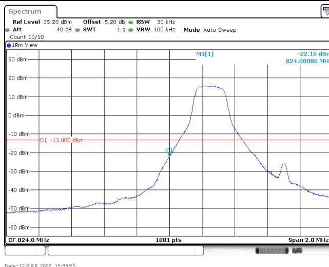
Band26_1.4MHz_QPSK_26797_6RB#0
