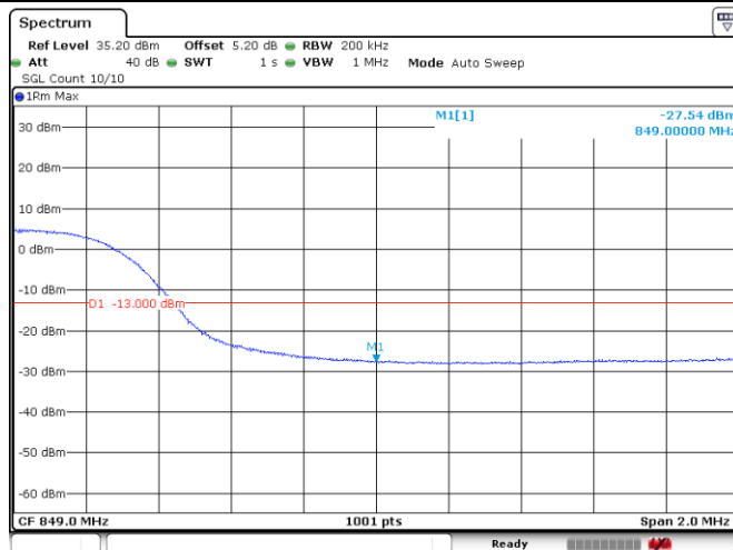
Band 26_15MHz_16QAM_26965_75RB#0
