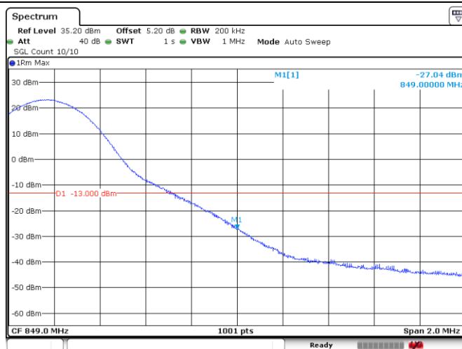
Band 26_15MHz_16QAM_26965_75RB#0
