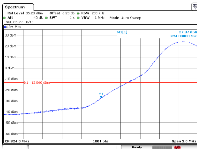
Band 26_15MHz_QPSK_26865_75RB#0
