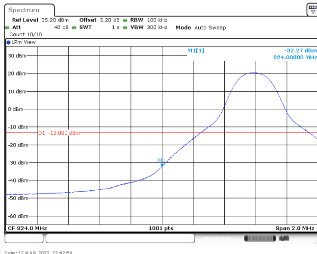
Band26_10MHz_QPSK_20450_50RB#0
