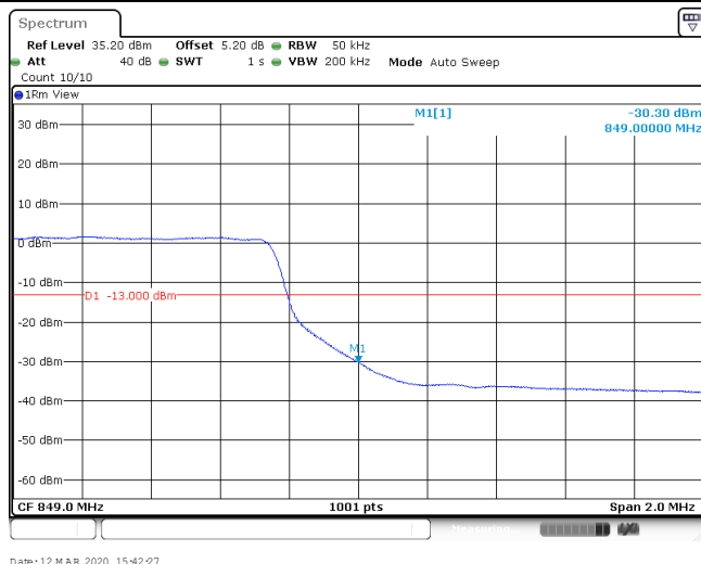
Band26_10MHz_QPSK_20450_1RB#0
