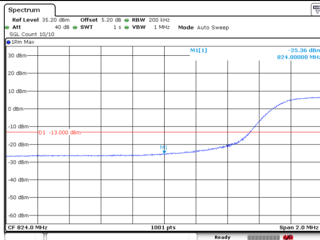
Band 26_15MHz_QPSK_26865_75RB#0
