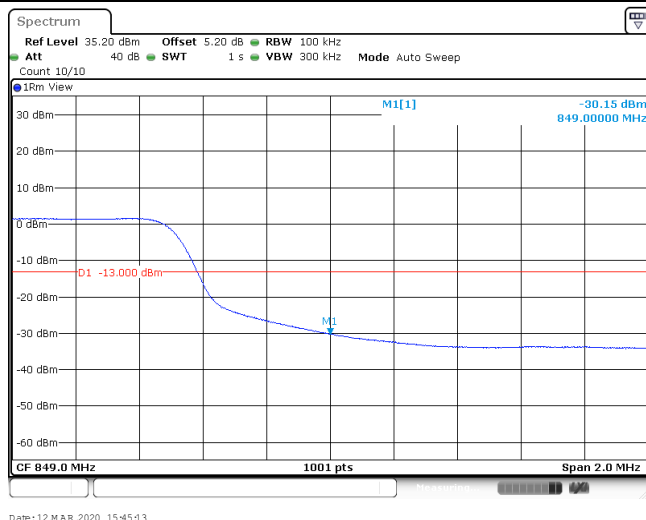
Band26_10MHz_16QAM_20450_1RB#0
