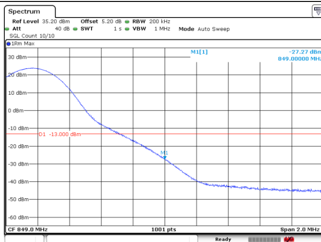
Band 26_15MHz_QPSK_26965_75RB#0
