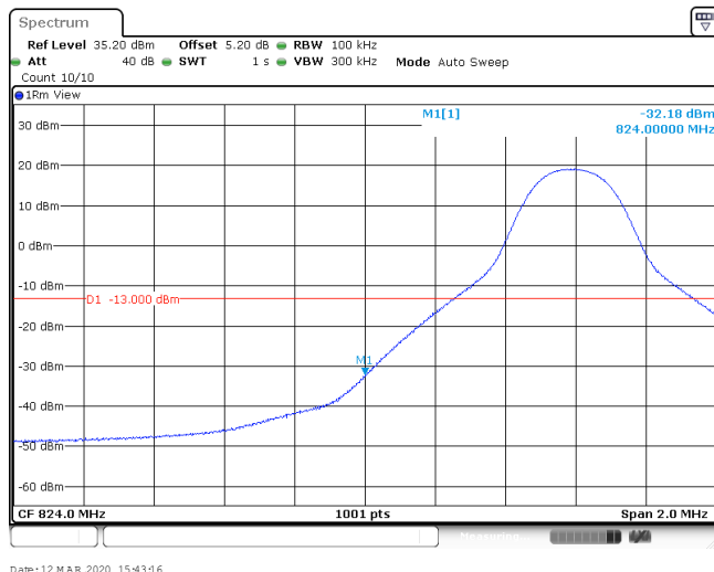
Band26_10MHz_16QAM_20450_50RB#0
