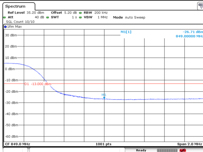
Band 26_15MHz_QPSK_26965_75RB#0
