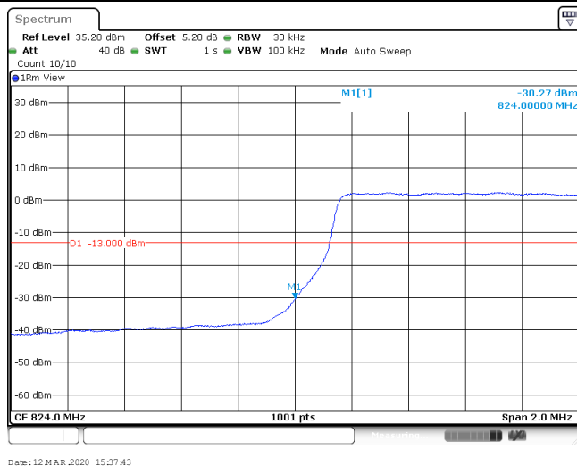
Band26_3MHz_16QAM_26915_1RB#14
