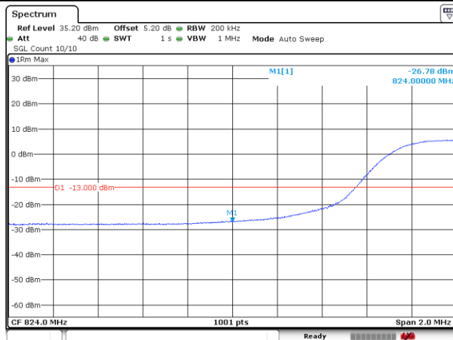
Band 26_15MHz_16QAM_26865_75RB#0
