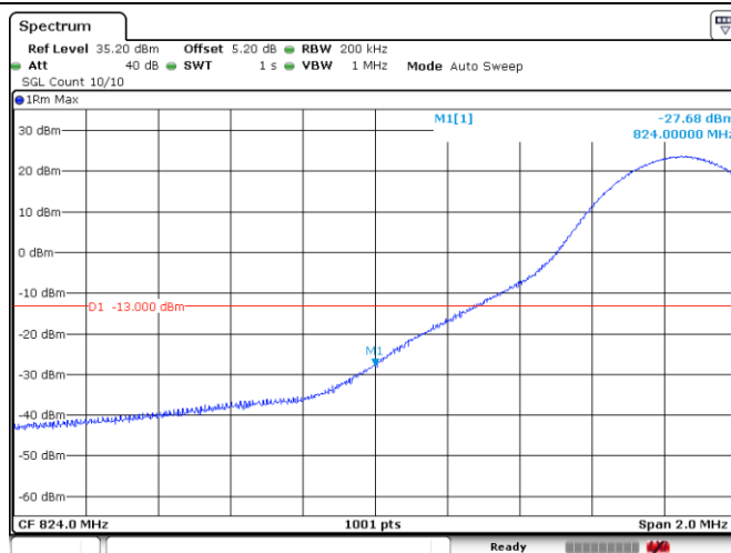
Band 26_15MHz_16QAM_26865_75RB#0
