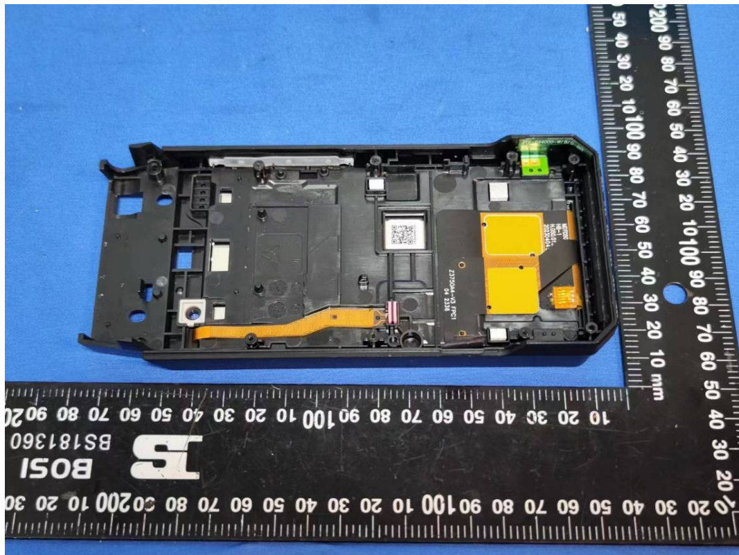
WiFi/Bluetooth Antenna
