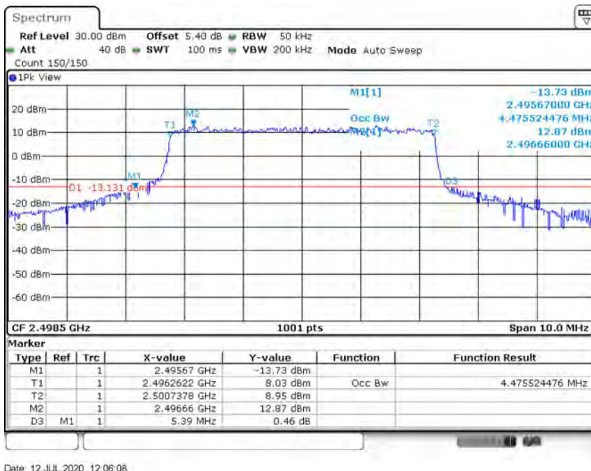
Band41-5MHz-QPSK-40620-25RB#0-4.476
