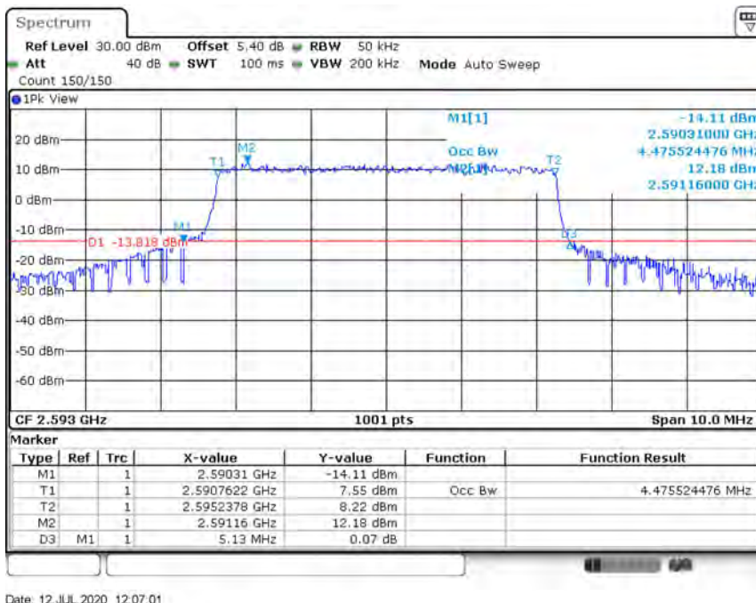
Band41-5MHz-QPSK-40620-25RB#0-4.476
