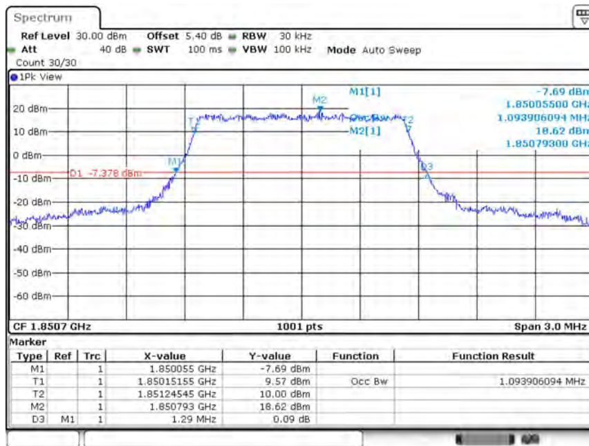
Band25-1.4MHz-QPSK-26047-6RB#0-1.094
