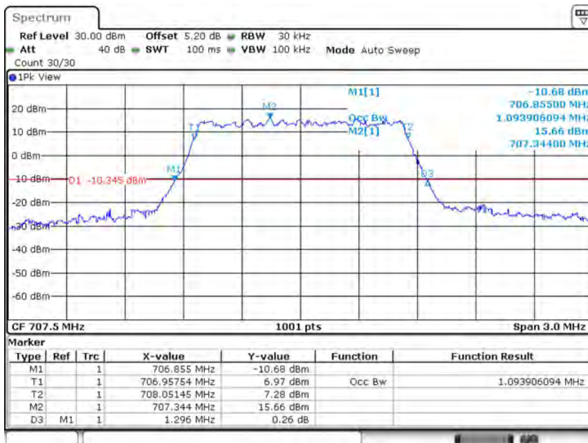
Band12-1.4MHz-QPSK-23095-6RB#0-1.094
