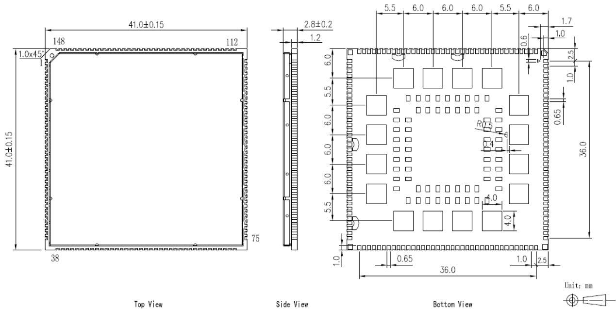
Figure 9-2 Structural dimension
