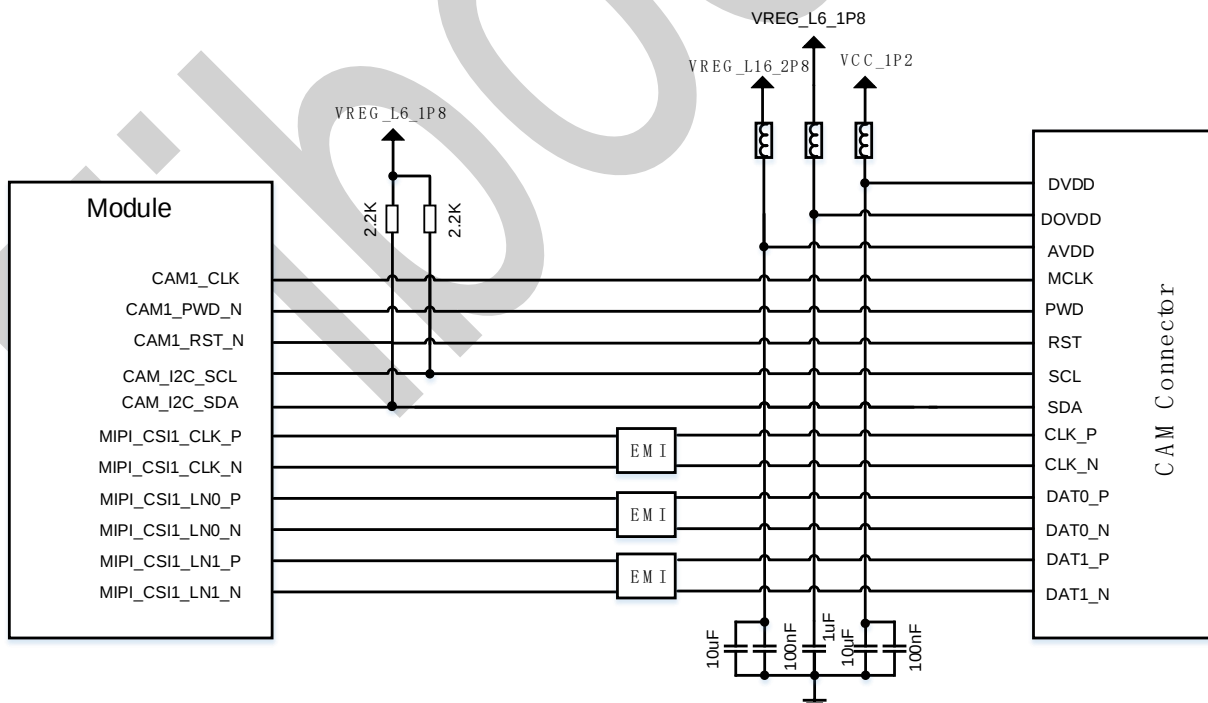
Figure 3-17 2 lane front camera reference design
