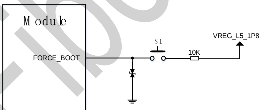
Figure 3-23 Force download reference design
