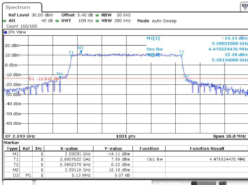
Band41-5MHz-QPSK-40620-25RB#0-4.476
