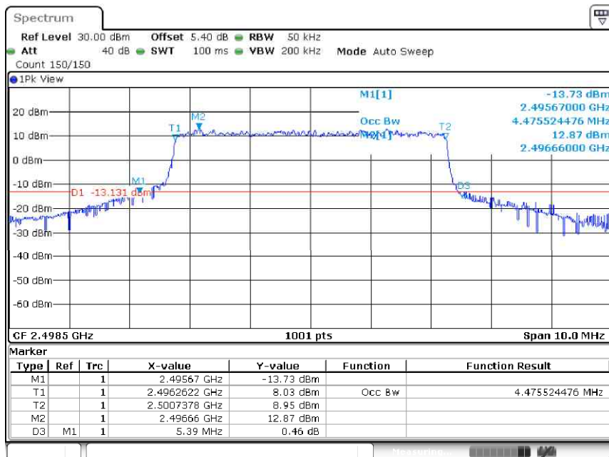
Band41-5MHz-QPSK-39675-25RB#0-4.476
