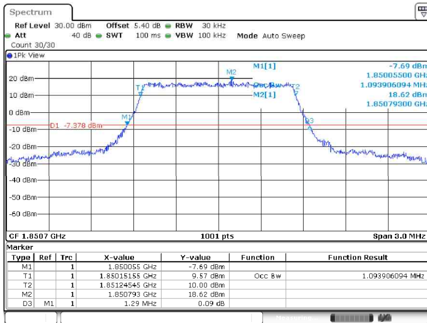
Band25-1.4MHz-QPSK-26047-6RB#0-1.094
