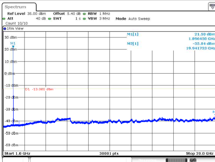
Band25-20MHz-16QAM-26590-1RB#0-Range2:1000~20000MHz
