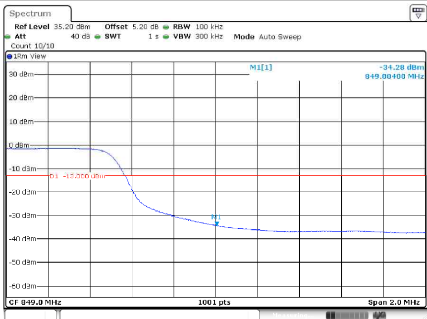
Band5-10MHz-16QAM-20600-50RB#0
