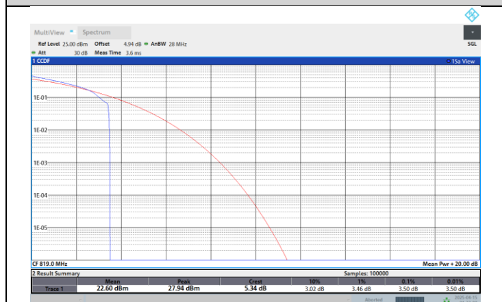
Band26-1.4MHz-16QAM-26783-1RB#0
