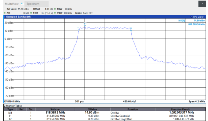
Band26-1.4MHz-16QAM-26697-6RB#0
