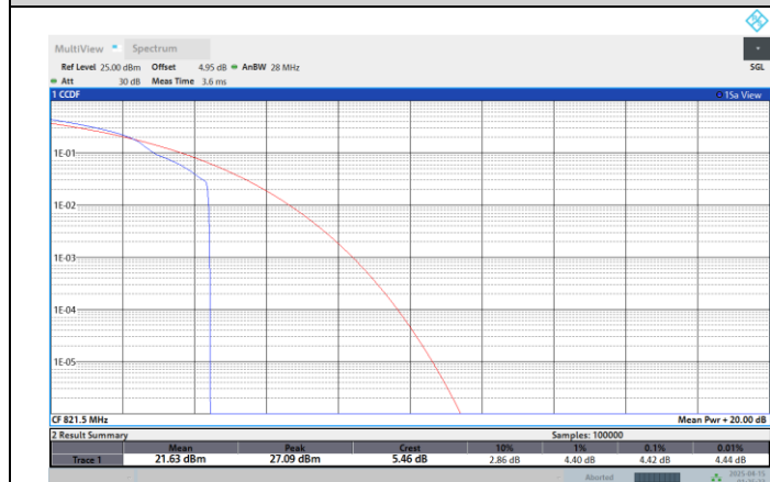
Band26-10MHz-QPSK-26740-1RB#0
