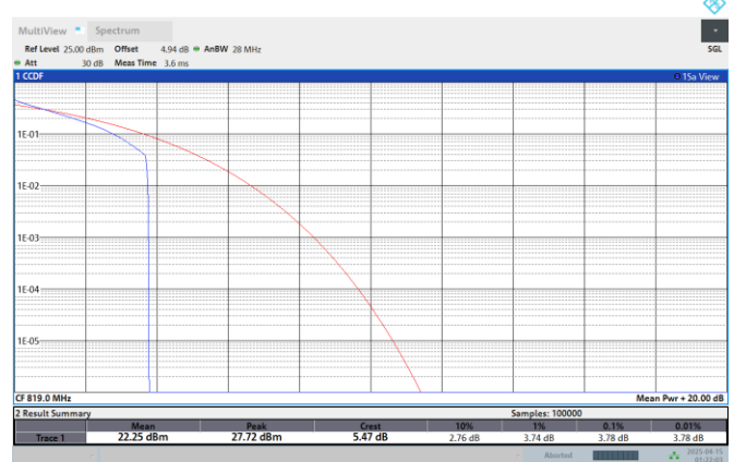
Band26-1.4MHz-QPSK-26783-6RB#0
