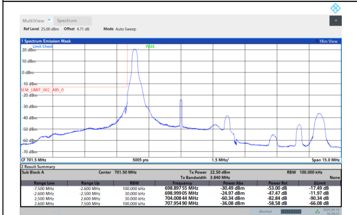
Band12-5MHz-QPSK-23155-1RB#24
