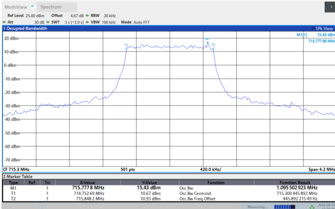
Band12-1.4MHz-16QAM-23095-6RB#0
