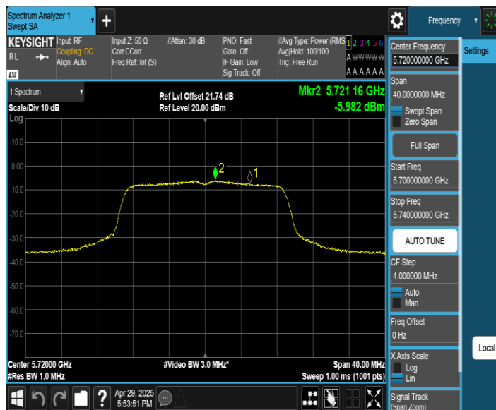
11AC20SISO_Ant1_5720_UNII-3
