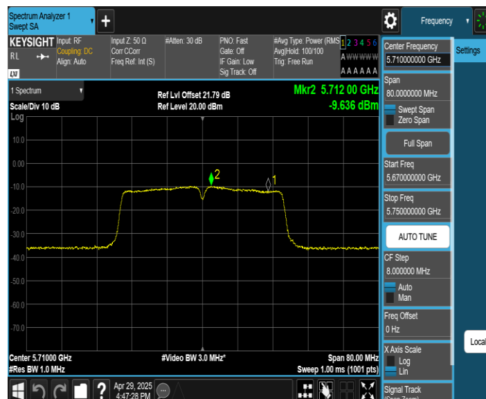
11N40SISO_Ant1_5710_UNII-3
