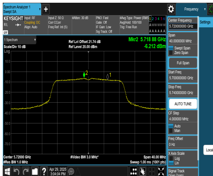
11N20SISO_Ant1_5720_UNII-3
