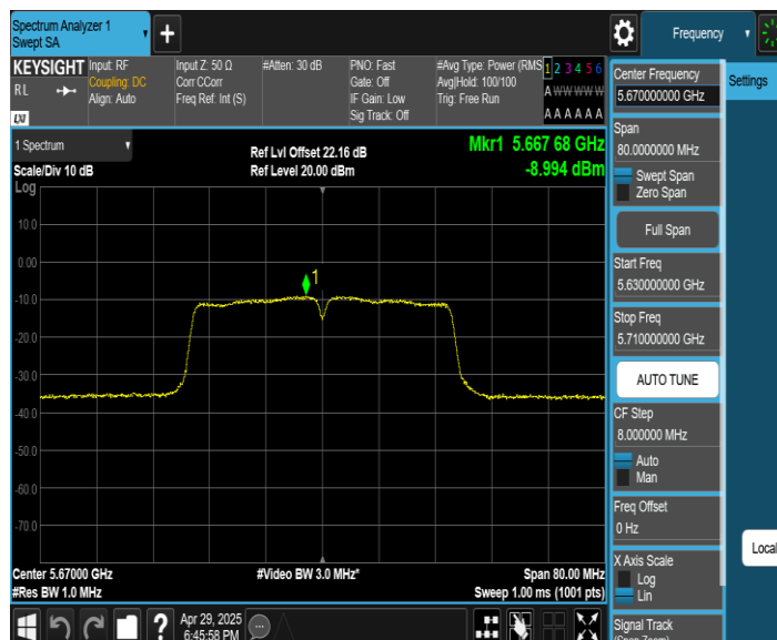
11AC40SISO_Ant1_5710_UNII-2C
