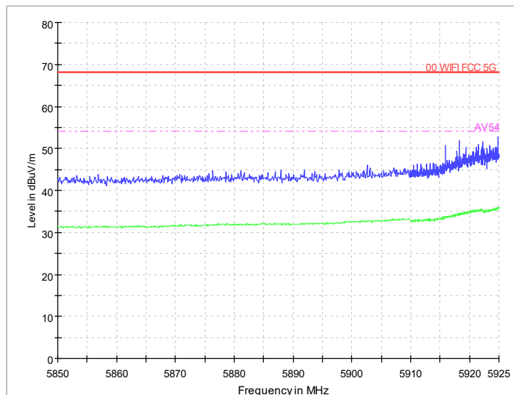
Radiated Emission Band Edge Channel No.:1 Test Mode: 802.11a Polarization: V
