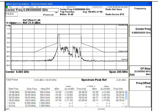
Mode:802.11ax HE40 Tone:26T Frequency:6885MHz Ant:Chain1
