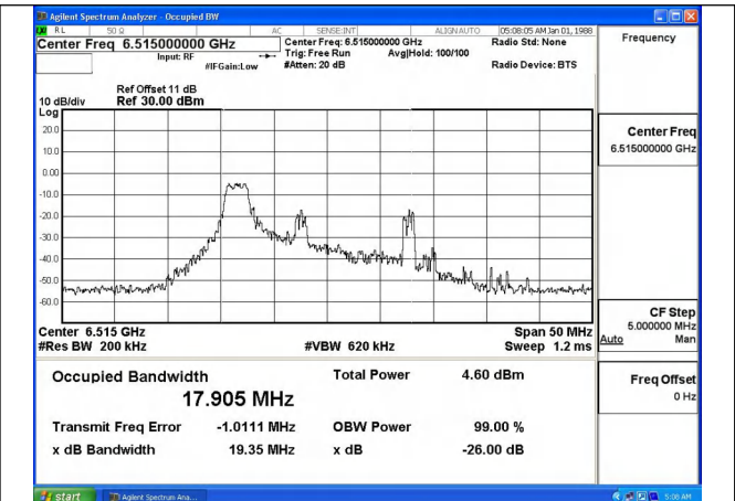
Mode:802.11ax HE20 Frequency:6515MHz Ant:Chain1
