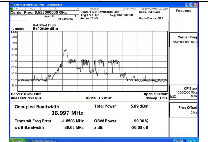
Mode:802.11ax HE40 Frequency:6525MHz Ant:Chain1
