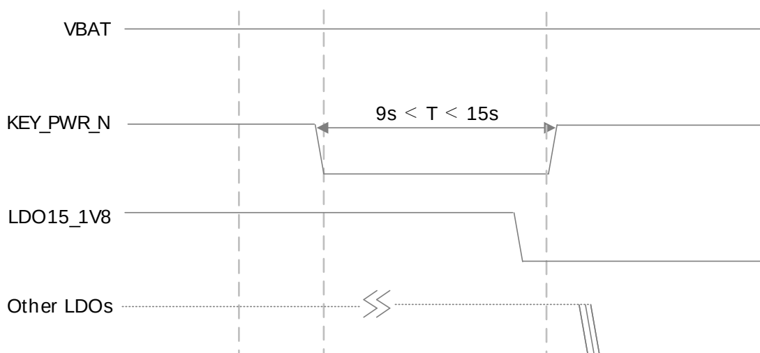
Figure 10. Power-off timing
