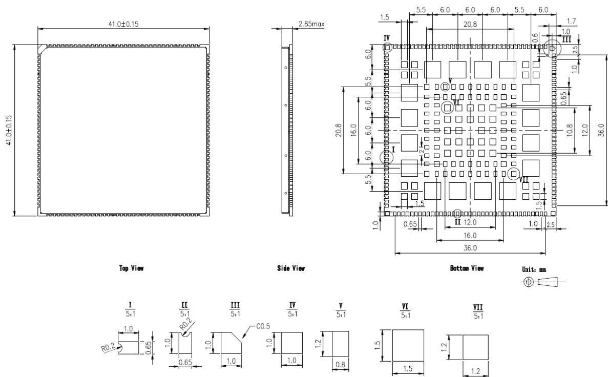
Figure 33. Structural dimensions
