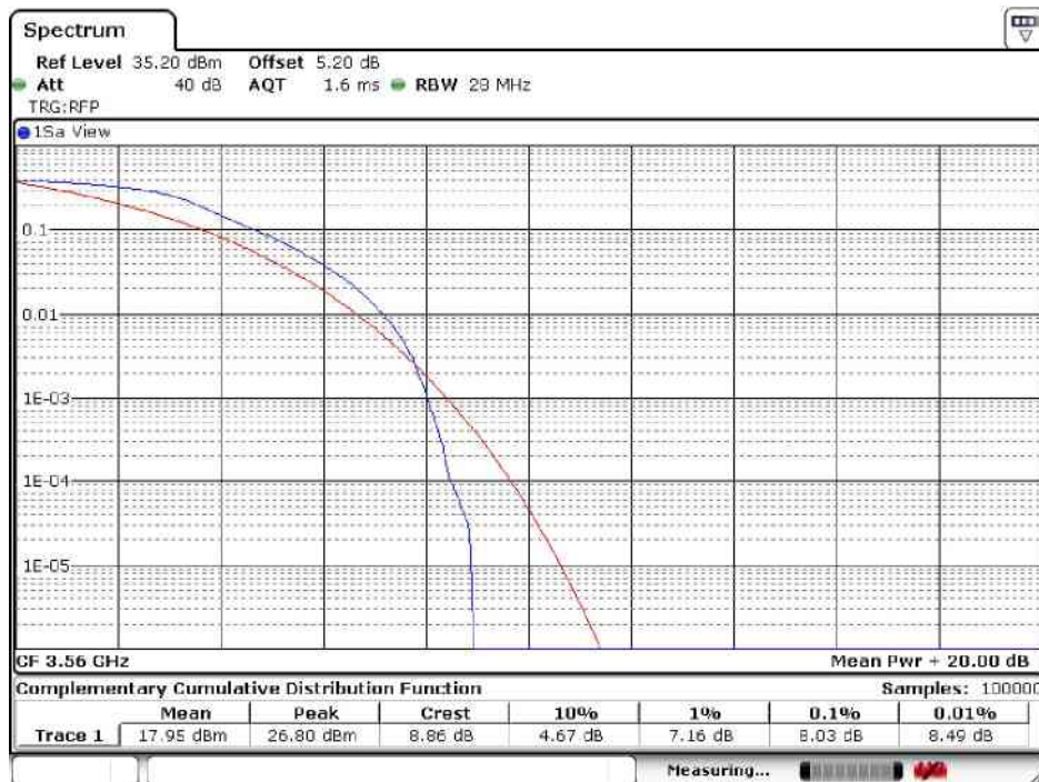
Band48-20MHz-QPSK-55340-100RB#0
