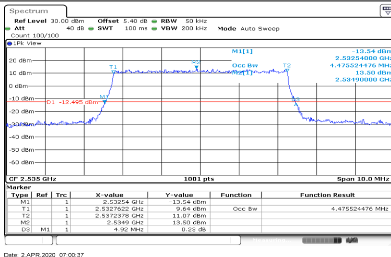
Band7-5MHz-QPSK-21425-25RB#0-4.476
