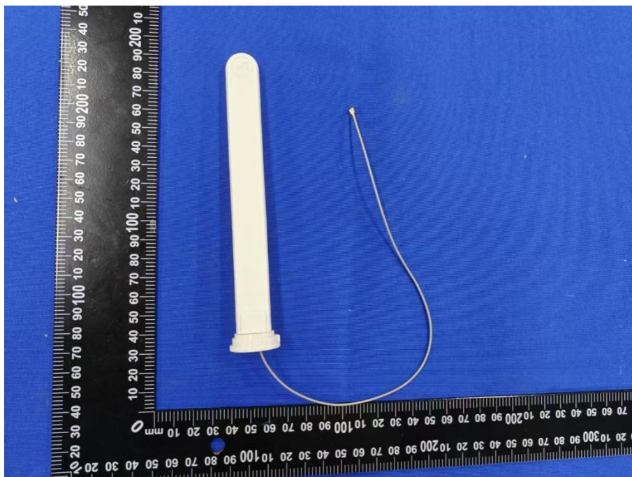
Accessory-TX Antenna_KIT-HK23-PT24-4G
