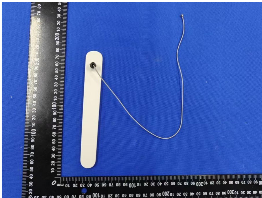
Accessory-TX Antenna _TQX-071427HK22-L
