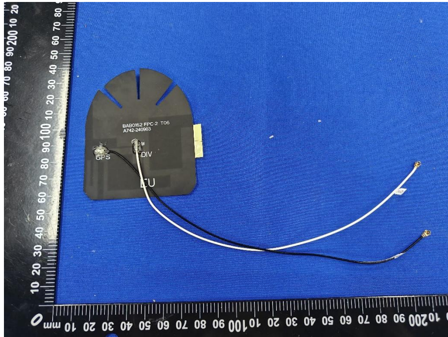
Accessory-DIV Antenna_F-0Y-31-0116-002-K0
