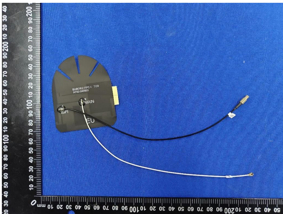
Accessory-TX Antenna _F-0Y-31-0116-001-K0
