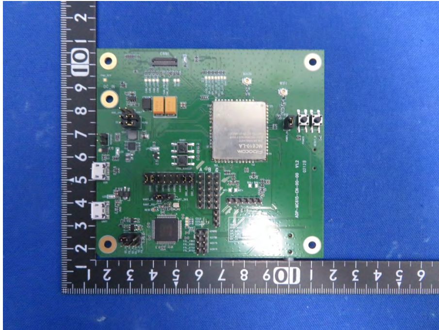
(1) Test Platform Photo
